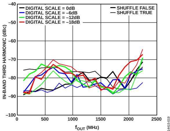
Figure 19. SFDR for In-Band Third Harmonic vs. f_{OUT} over Digital Scale
