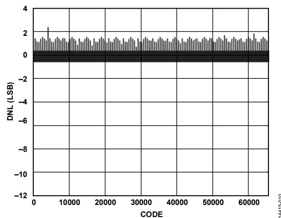
Figure 10. DNL, I_{OUTFS} = 40 mA
