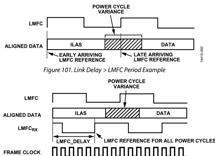
Figure 102. LMFC_DELAY_x to Compensate for Link Delay > LMFC
