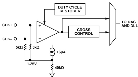
Figure 131. Clock Input
