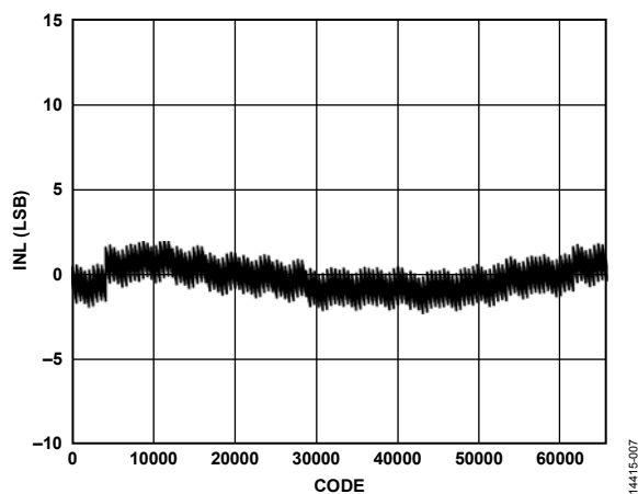
Figure 7. INL, I_{OUTFS} = 40 mA
