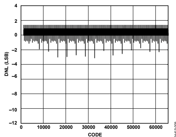
Figure 9. DNL, I_{OUTFS} = 30 mA
