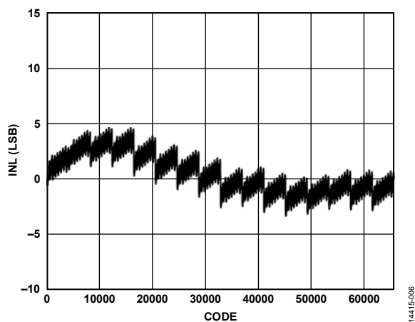
Figure 6. INL, I_{OUTFS} = 30 mA
