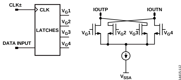
Figure 126. Quad-Switch Architecture
