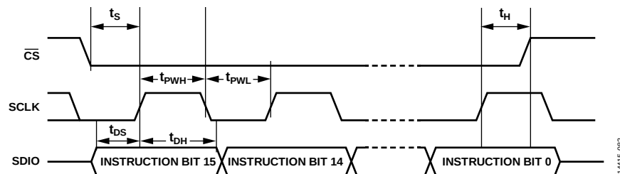
Figure 89. Timing Diagram for Serial Port Register Write
