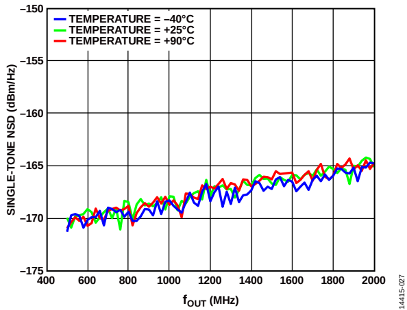
Figure 29. Single-Tone NSD Measured at 70 MHz vs. f_{OUT} over Temperature
