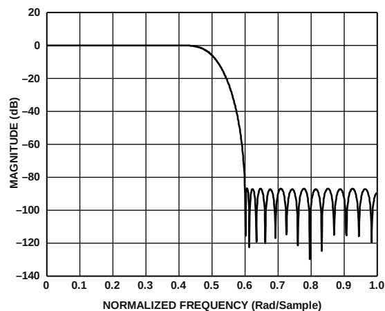
Figure 110. First 2x Half-Band 80% Filter Response
