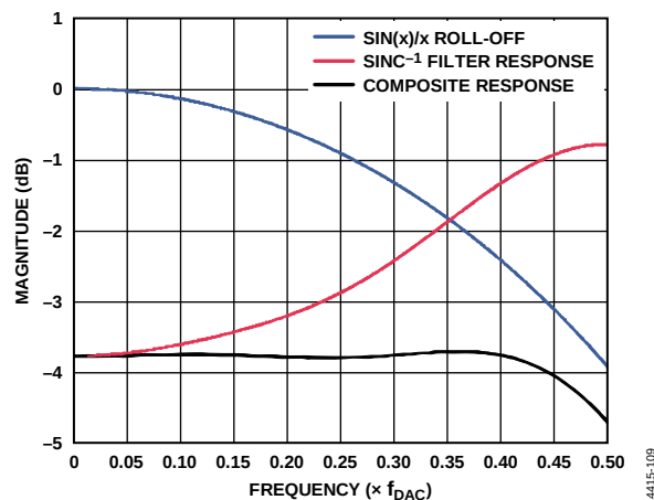
Figure 119. Responses of \sin(x)/x Roll-Off, the \text{Sinc}^{-1} Filter, and the Composite of the Two
