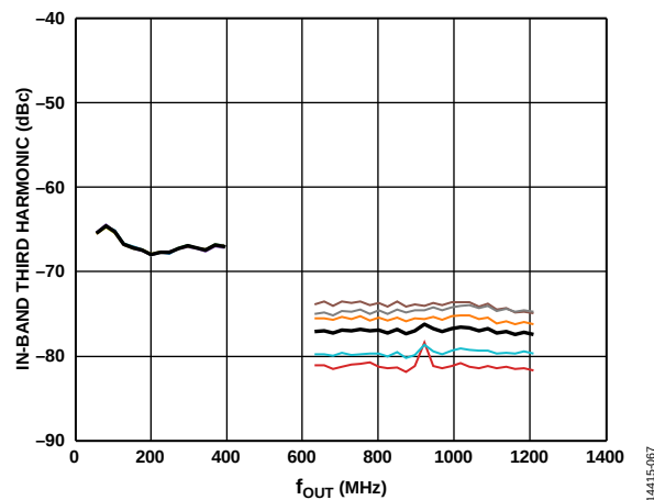
Figure 74. In-Band Third Harmonic vs. f_{OUT} Performance for One DOCSIS Carrier
