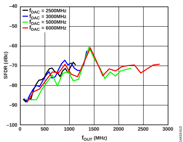
Figure 13. SFDR vs. f_{OUT} over f_{DAC}
