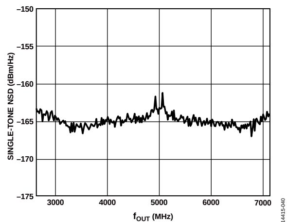
Figure 43. Single-Tone NSD vs. f_{OUT}
