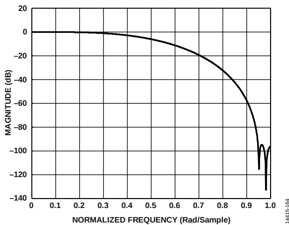
Figure 116. Fourth 2x Half-Band 11.25% Filter Response
