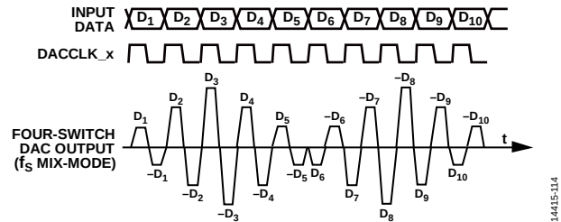
Figure 128. Mix-Mode Waveform
