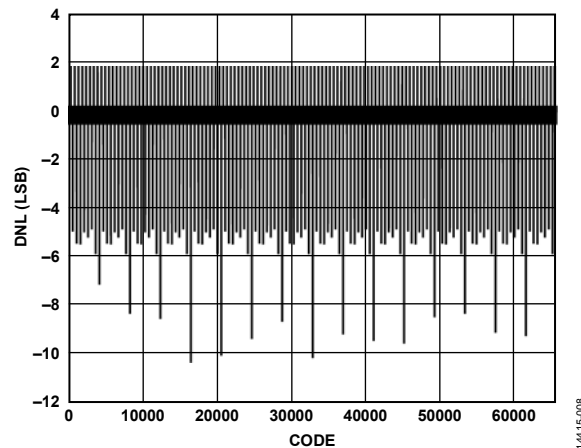
Figure 8. DNL, I_{OUTFS} = 20 mA
