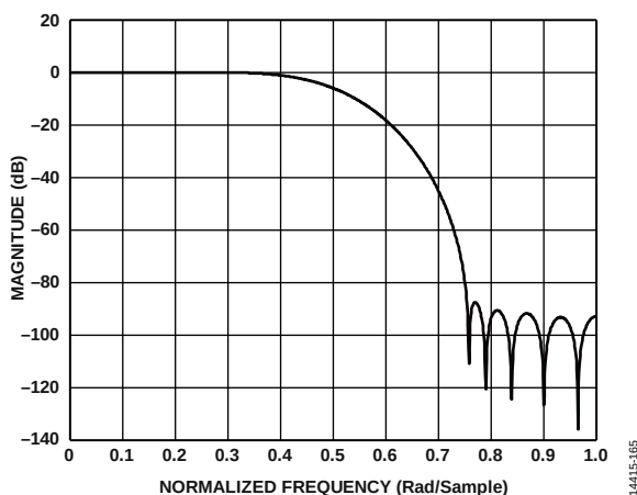
Figure 117. FIR85 2x Half-Band 45% Filter Response
