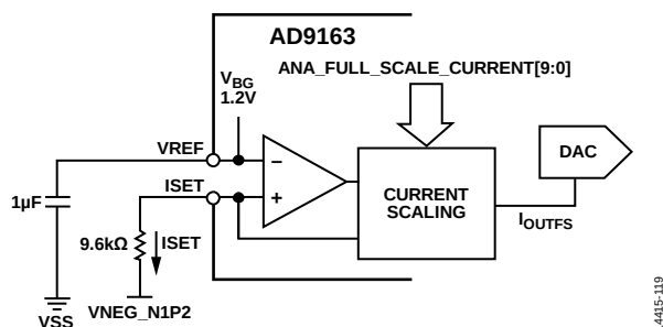
Figure 133. Voltage Reference Circuit
