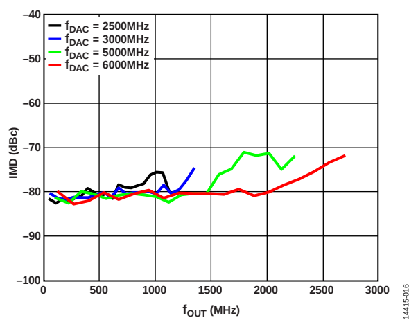
Figure 16. IMD vs. f_{OUT} over f_{DAC}
