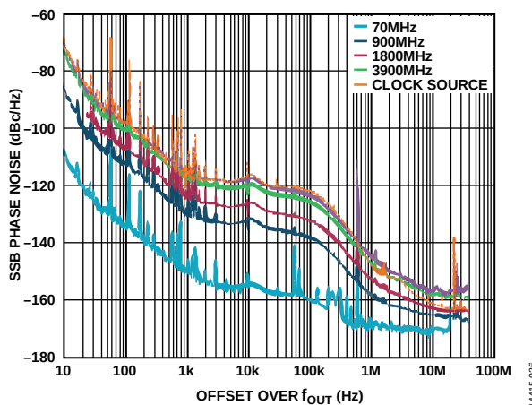
Figure 40. SSB Phase Noise vs. Offset over f_{OUT} , f_{DAC} = 6000 \text{ MSPS}
