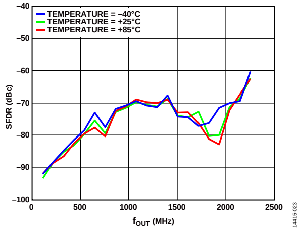
Figure 23. SFDR vs. f_{OUT} over Temperature
