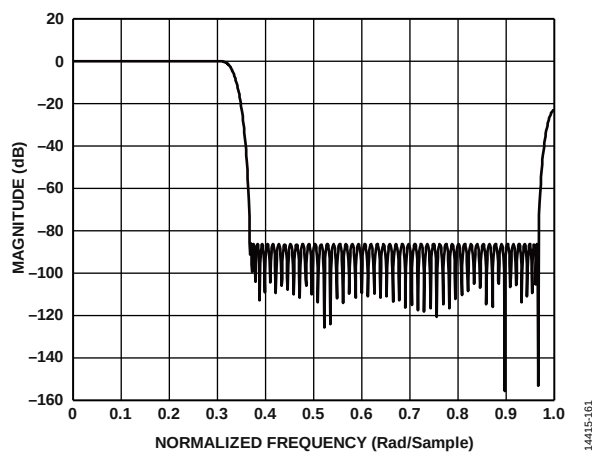
Figure 113. 3x Third-Band 90% Filter Response
