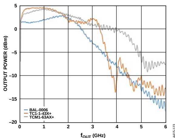
Figure 138. Measured DAC Output Response; f_{DAC} = 6 GSPS
