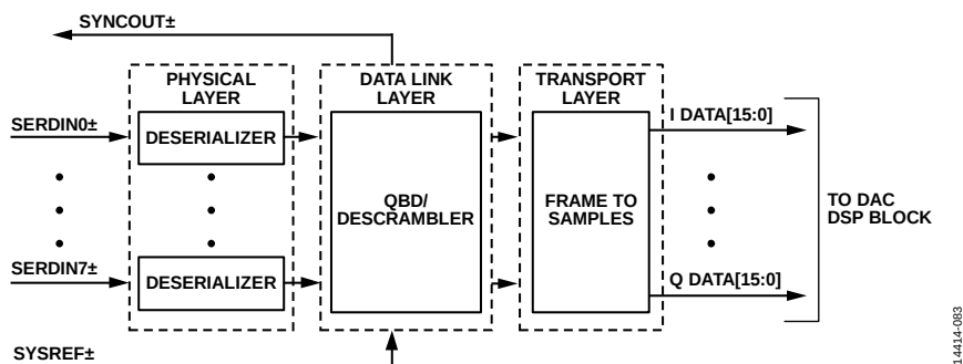
Figure 91. Functional Block Diagram of Serial Link Receiver
