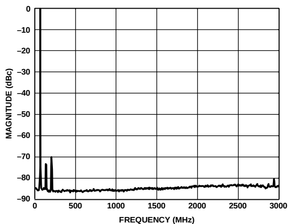
Figure 60. Single Carrier at 70 MHz Output
