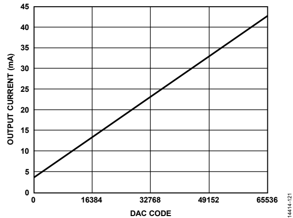
Figure 138. Gain Curve for ANA\_FULL\_SCALE\_CURRENT[9:0] = 1023 , DAC Offset = 3.8 mA
