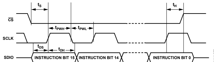
Figure 90. Timing Diagram for Serial Port Register Write
