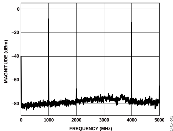
Figure 45. Single-Tone Spectrum at f_{OUT} = 4000\text{ MHz}
