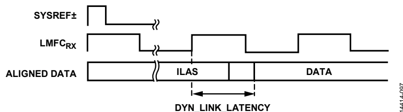
Figure 106. DYN_LINK_LATENCY_x Illustration
