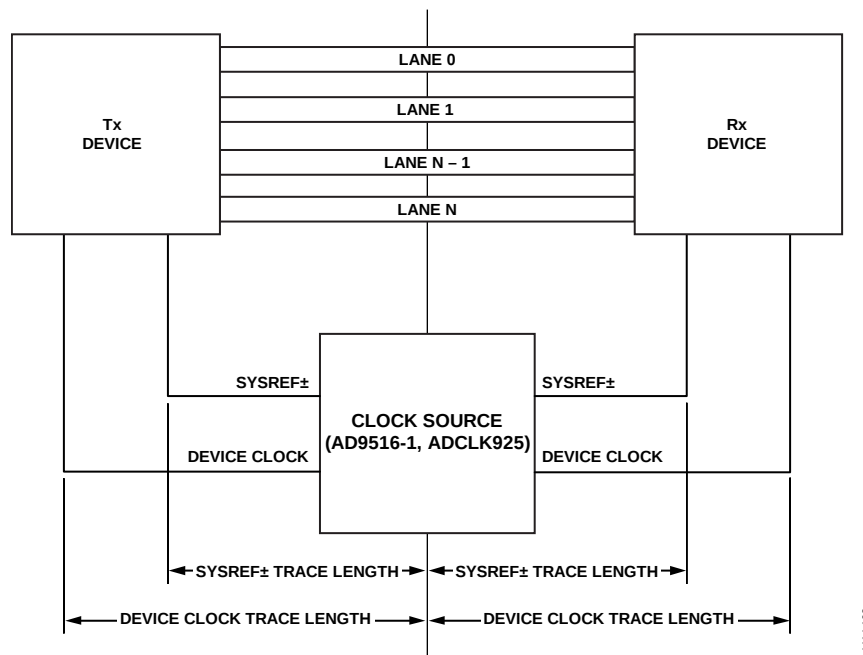
Figure 127. SYSREF± Signal and Device Clock Trace Length
