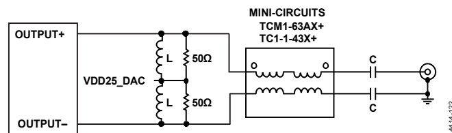
Figure 140. Recommended Transformer for Wideband Applications with Upper Bandwidths of up to 5 GHz
