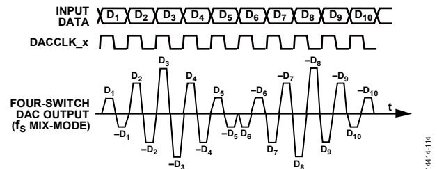
Figure 130. Mix-Mode Waveform
