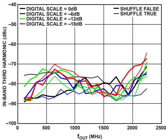
Figure 20. SFDR for In-Band Third Harmonic vs. f_{OUT} over Digital Scale
