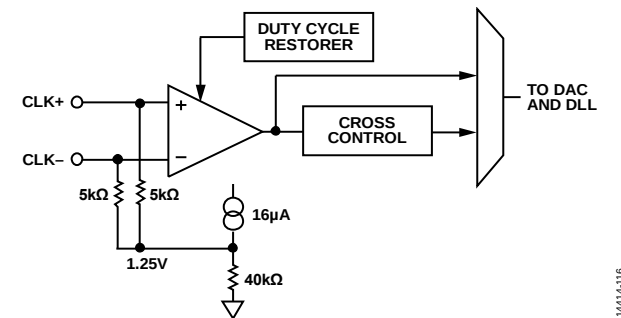
Figure 133. Clock Input
