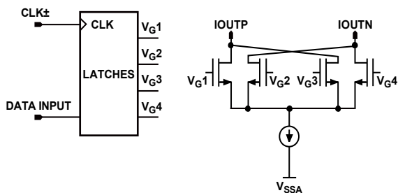
Figure 128. Quad-Switch Architecture
