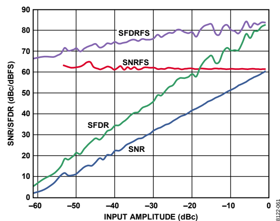
Figure 15. AD9204-80 SNR/SFDR vs. Input Amplitude (AIN) with f_{IN} = 9.7 MHz
