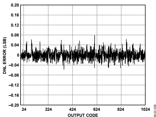
Figure 14. AD9204-80 DNL with f_{IN} = 9.7 MHz
