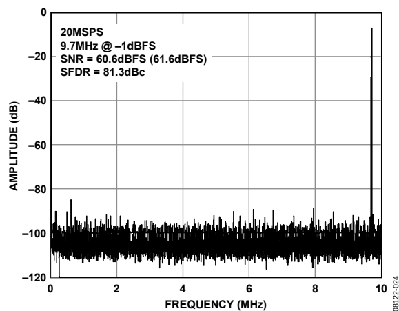
Figure 26. AD9204-20 Single-Tone FFT with f_{IN} = 9.7 MHz
