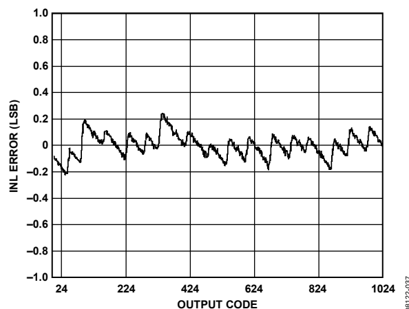
Figure 17. AD9204-80 INL with f_{IN} = 9.7 MHz
