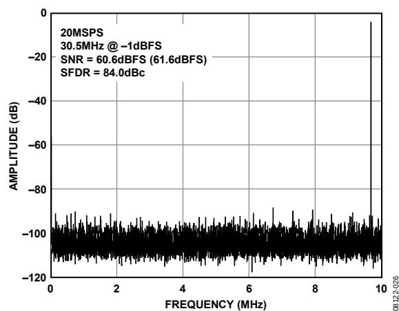
Figure 27. AD9204-20 Single-Tone FFT with f_{IN} = 30.5 MHz
