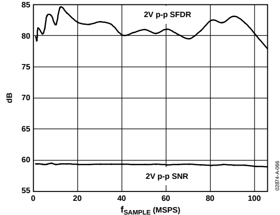
Figure 14. AD9215-105 SNR/SFDR vs. f_{SAMPLE} , f_{IN} = 10.3\text{ MHz}
