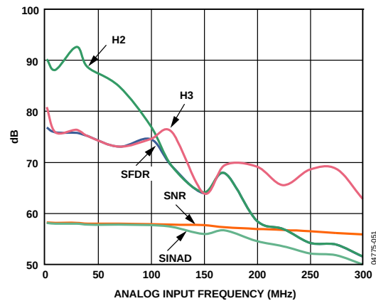
Figure 13. Analog Input Frequency Sweep, A_{IN} = -0.5 dBFS, f_s = 80 MSPS ( -80 Grade)
