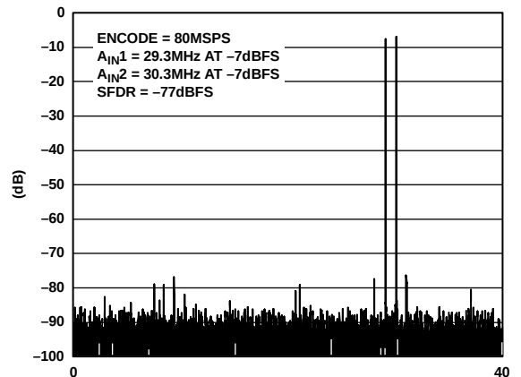
Figure 25. Two-Tone Intermodulation Distortion ( 29.3 \text{ MHz} and 30.3 \text{ MHz} ; 1 \text{ V p-p} , FS = 80 \text{ MSPS} )
