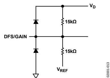
Figure 13. DFS/Gain Input
