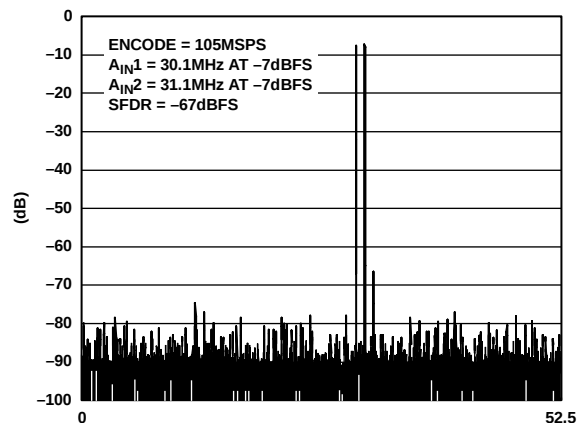
Figure 24. Two-Tone Intermodulation Distortion ( 30.1 \text{ MHz} and 31.1 \text{ MHz} ; 1 \text{ V p-p} , FS = 105 \text{ MSPS} )
