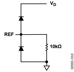
Figure 10. Reference Inputs
