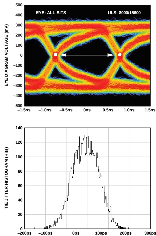
Figure 78. Data Eye for LVDS Outputs in ANSI-644 Mode with 100 \Omega Termination on and Trace Lengths Greater than 24 Inches on Standard FR-4, AD9222-65
