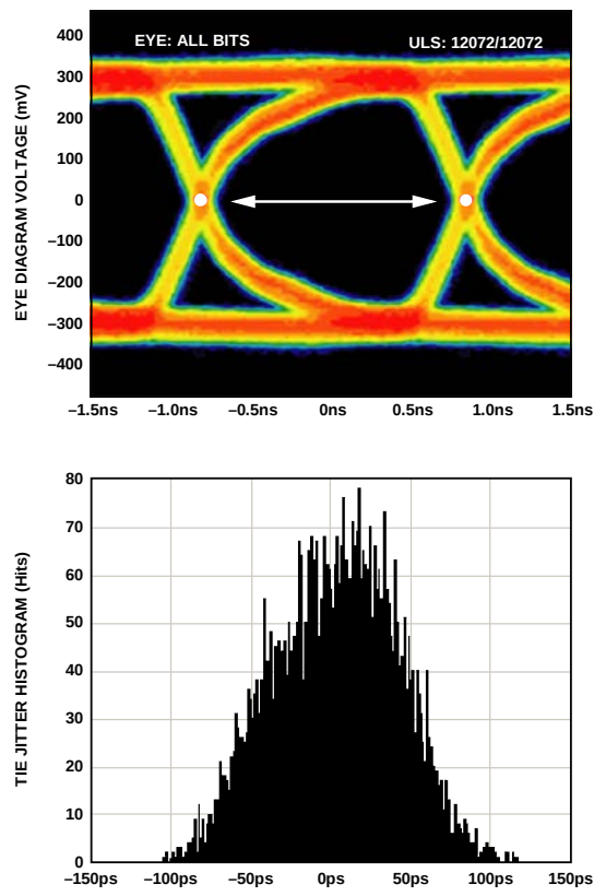
Figure 77. Data Eye for LVDS Outputs in ANSI-644 Mode with 100 \Omega Termination on and Trace Lengths Greater than 24 Inches on Standard FR-4, AD9222-50
