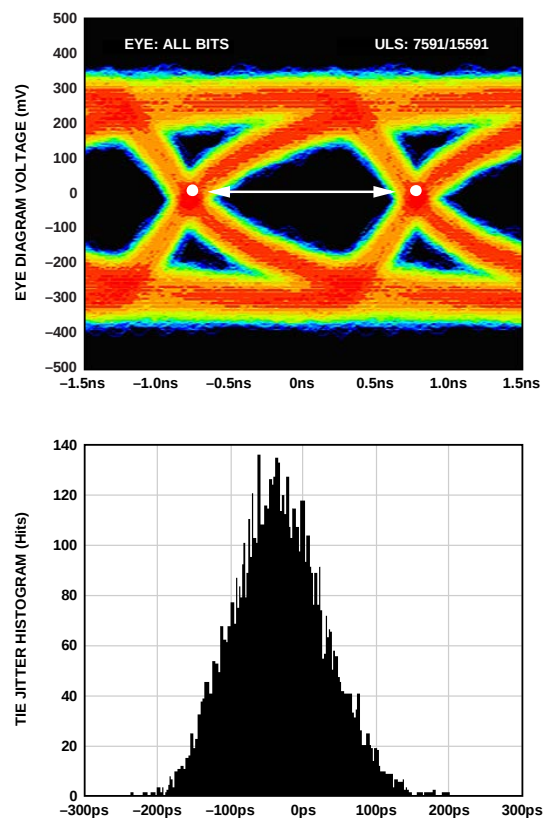
Figure 76. Data Eye for LVDS Outputs in ANSI-644 Mode with Trace Lengths Greater than 24 Inches on Standard FR-4, AD9222-65
