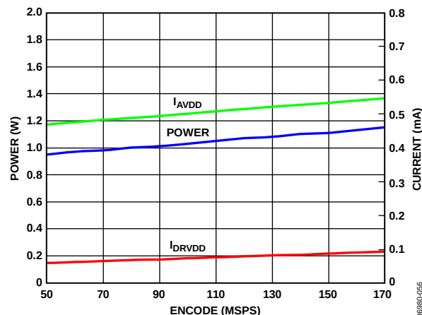
Figure 58. Supply Current vs. Encode for f_{IN} = 84.3 MHz, f_{SAMPLE} = 170 MSPS
