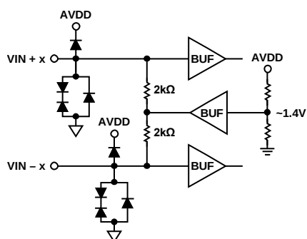
Figure 36. Analog Inputs
