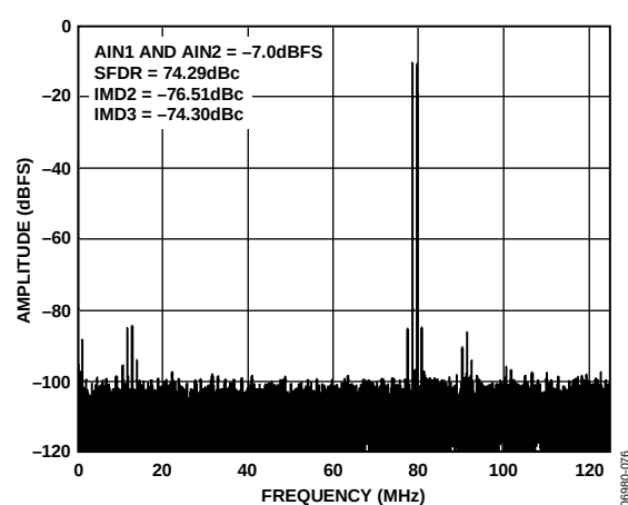
Figure 21. Two-Tone 32k FFT with f_{IN1} = 170.2 MHz and f_{IN2} = 171.3 MHz, f_{SAMPLE} = 250 MSPS
