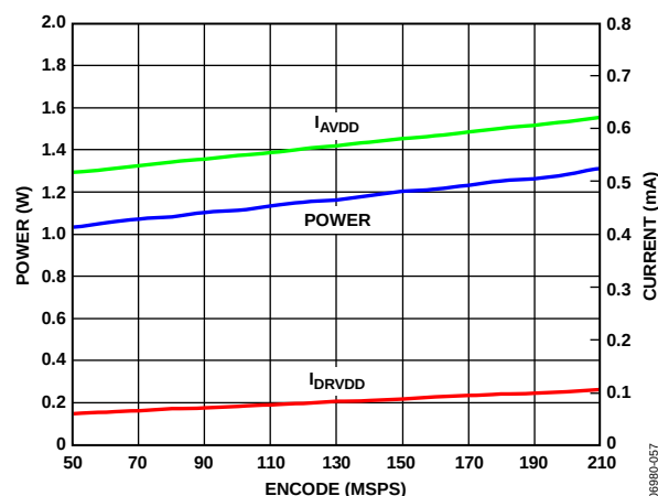
Figure 59. Supply Current vs. Encode for f_{IN} = 84.3 MHz, f_{SAMPLE} = 210 MSPS
