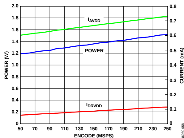
Figure 60. Supply Current vs. Encode for f_{IN} = 84.3 MHz, f_{SAMPLE} = 250 MSPS
