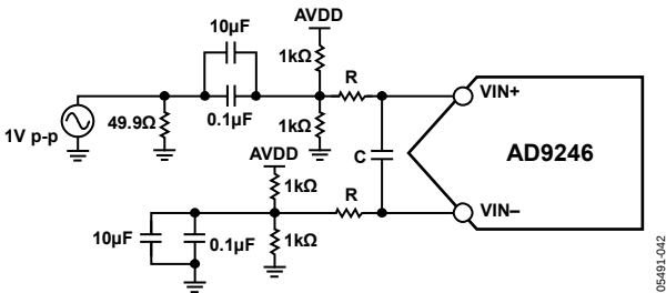
Figure 39. Single-Ended Input Configuration
