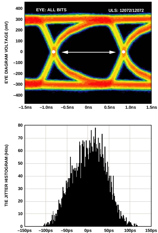
Figure 50. Data Eye for LVDS Outputs in ANSI-644 Mode with 100 \Omega Termination On and Trace Lengths Greater Than 24 Inches on Standard FR-4
