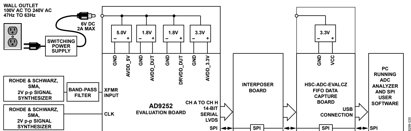
Figure 58. Evaluation Board Connection
