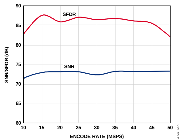
Figure 19. SNR/SFDR vs. f_{SAMPLE} , f_{IN} = 10.3 MHz, AD9252-50
