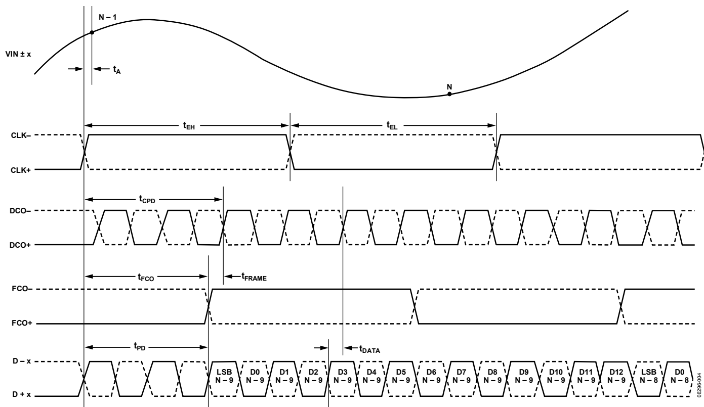
Figure 4. 14-Bit Data Serial Stream, LSB First
