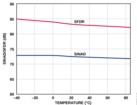
Figure 26. SINAD/SFDR vs. Temperature, f_{IN} = 19.7 MHz, f_{SAMPLE} = 50 MSPS
