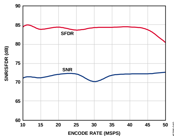
Figure 20. SNR/SFDR vs. f_{SAMPLE} , f_{IN} = 19.7 MHz, AD9252-50
