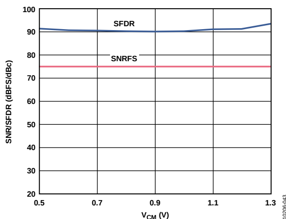
Figure 44. SNR/SFDR vs. Common-Mode Voltage, f_{IN} = 9.7 \text{ MHz} , f_{SAMPLE} = 65 \text{ MSPS}
