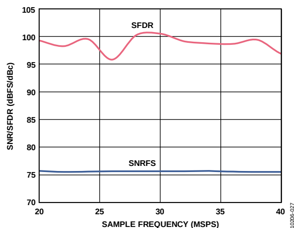
Figure 28. SNR/SFDR vs. Encode, f_{IN} = 19.7 MHz, CLK Divider = 4
