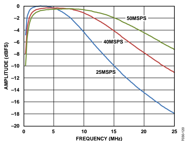
Figure 17. Antialiasing Filter (AAF) Pass-Band Response, LPF\text{ Cutoff} = 1 \times (1/3) \times f_{SAMPLE}
