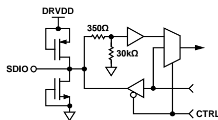
Figure 17. SDIO
