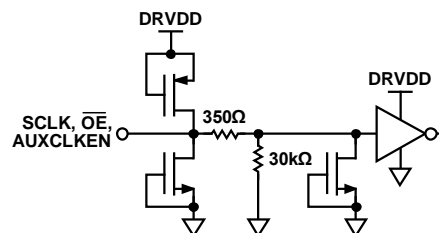
Figure 16. SCLK, \overline{OE}
