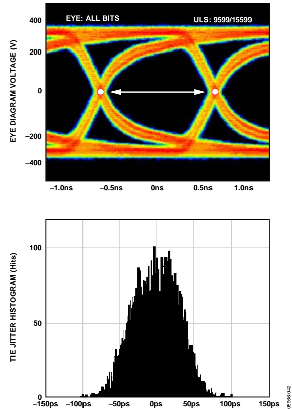
Figure 52. Data Eye for LVDS Outputs in ANSI-644 Mode with 100 \Omega Internal Termination on and Trace Lengths Greater than 24 Inches on Standard FR-4, External 100 \Omega Far Termination Only
