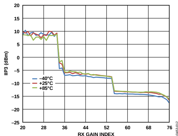
Figure 12. Third-Order Input Intercept Point (IIP3) vs. RX Gain Index, f_1 = 1.45 MHz, f_2 = 2.89 MHz, GSM Mode
