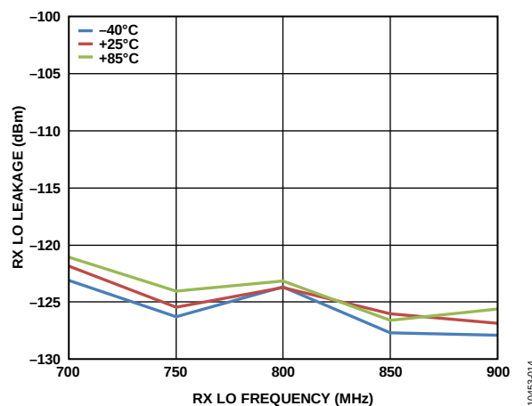
Figure 14. RX Local Oscillator (LO) Leakage vs. RX LO Frequency
