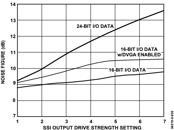
Figure 35. NF vs. SSI Output Drive Strength ( V_{DDX} = 3.0\text{ V} , F_{CLK} = 18\text{ MSPS} , BW = 75\text{ kHz} )
