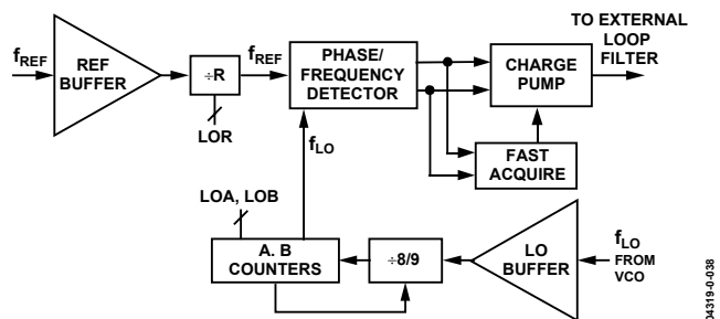
Figure 38. LO Synthesizer
