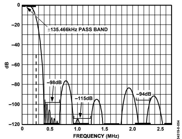
Figure 53. Decimation Filter Frequency Response for f_{OUT} = 541.666 kSPS ( f_{CLK} = 26 MHz, OSR = 48)
