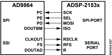
Figure 37. Example of AD9864 and ADSP-2153x Interface
