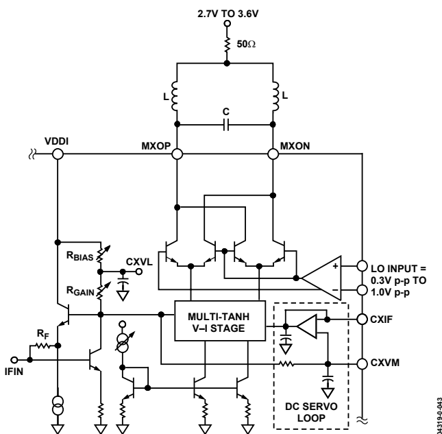
Figure 43. Simplified Schematic of AD9864's LNA/Mixer
