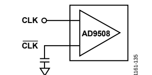
Figure 37. Typical 2.5 V or 3.3 V CMOS Configurations for Short Trace Lengths
