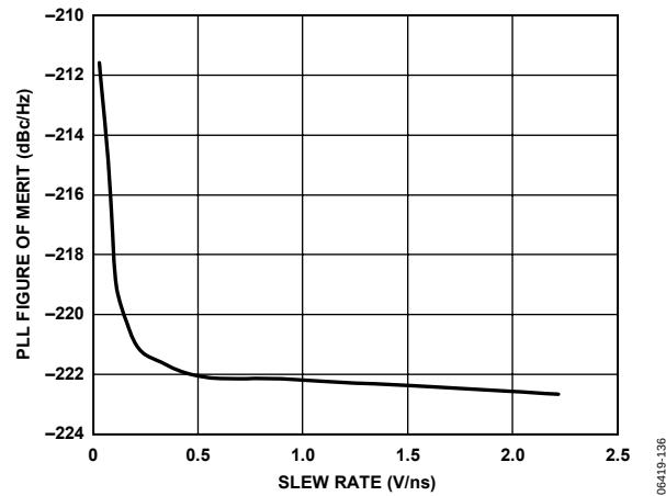
Figure 14. PLL Figure of Merit (FOM) vs. Slew Rate at \text{REFIN}/\overline{\text{REFIN}}
