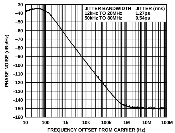
Figure 8. Phase Noise ( f_{REF} = 8 \text{ kHz} , f_{OUT1} = 155.52 \text{ MHz} )
