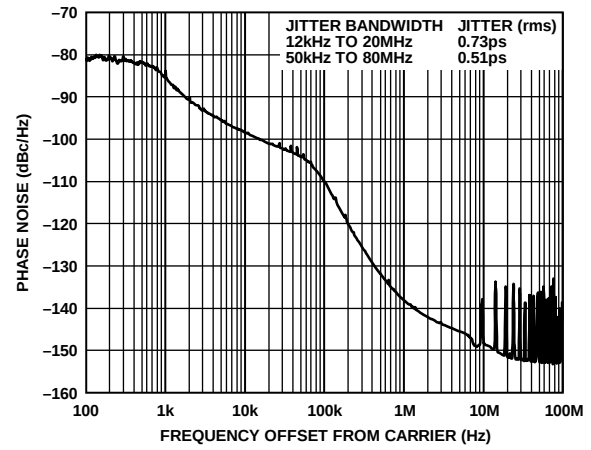
Figure 6. Phase Noise ( f_{REF} = 77.76 \text{ MHz} , f_{OUT1} = 622.08 \text{ MHz} )
