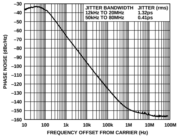
Figure 4. Phase Noise ( f_{REF} = 25 \text{ MHz} , f_{OUT1} = 156.25 \text{ MHz} )
