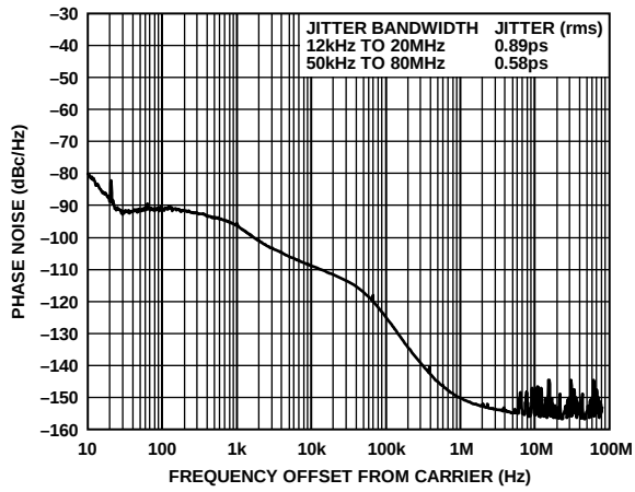
Figure 3. Phase Noise ( f_{REF} = 25 \text{ MHz} , f_{OUT1} = 125 \text{ MHz} )
