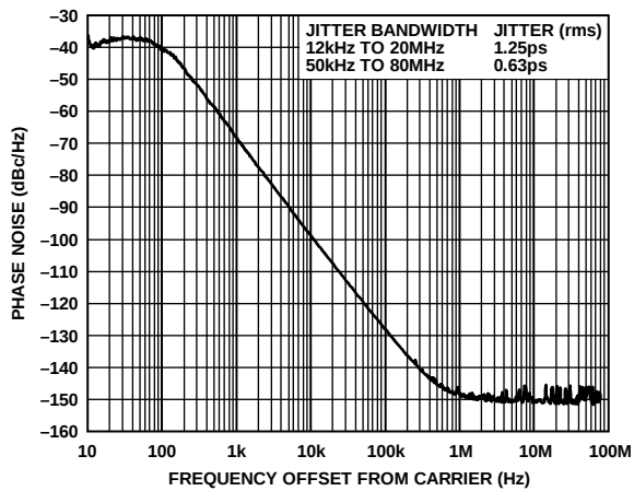
Figure 5. Phase Noise ( f_{REF} = 61.44 \text{ MHz} , f_{OUT1} = 122.88 \text{ MHz} )
