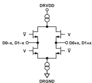
Figure 49. Equivalent Digital Output Circuit
