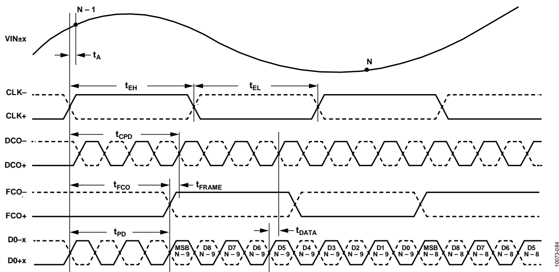
Figure 7. Wordwise DDR, One-Lane, 1× Frame, 10-Bit Output Mode
