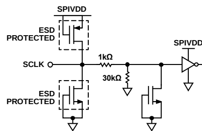
Figure 58. SCLK Input
