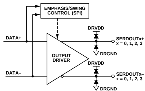
Figure 56. Digital Outputs
