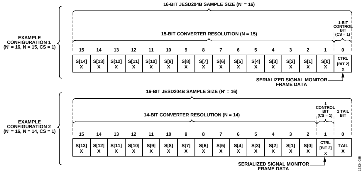
Figure 85. Signal Monitor Control Bit Locations
