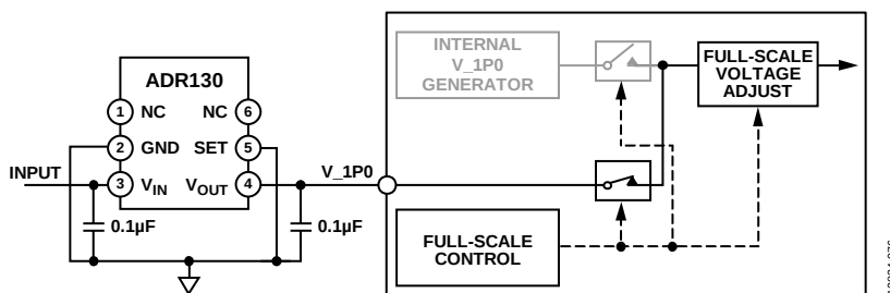
Figure 76. External Reference Using AD130
