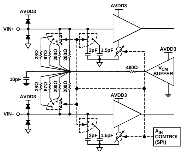
Figure 53. Analog Inputs
