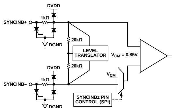
Figure 57. SYNCINB± Inputs
