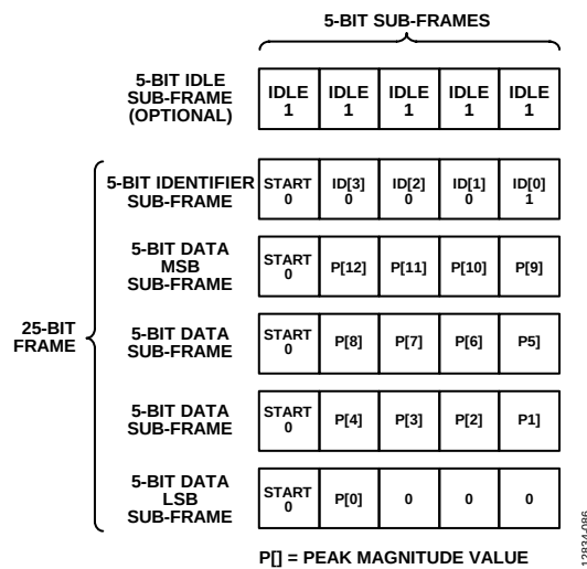
Figure 86. SPORT over JESD204B Signal Monitor Frame Data
