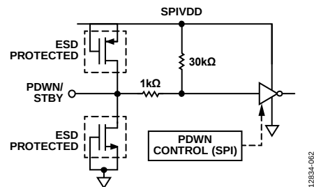
Figure 62. PDWN/STBY Input
