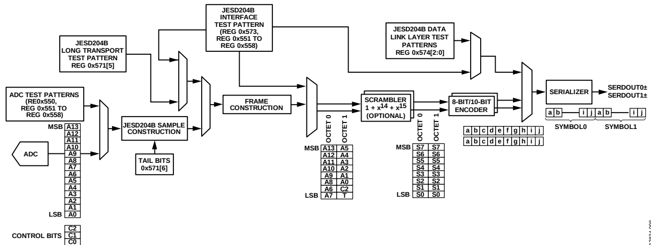
Figure 98. ADC Output Data Path Showing Data Framing
