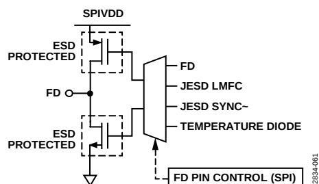
Figure 61. FD Outputs
