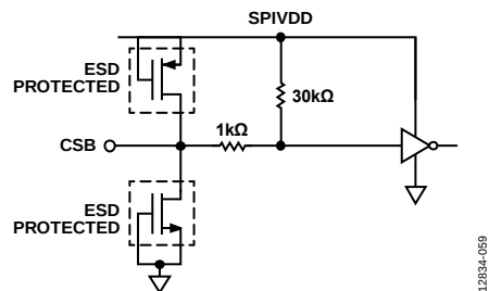
Figure 59. CSB Input
