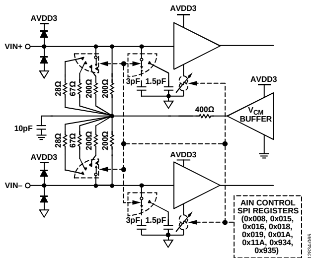
Figure 65. Analog Input Controls
