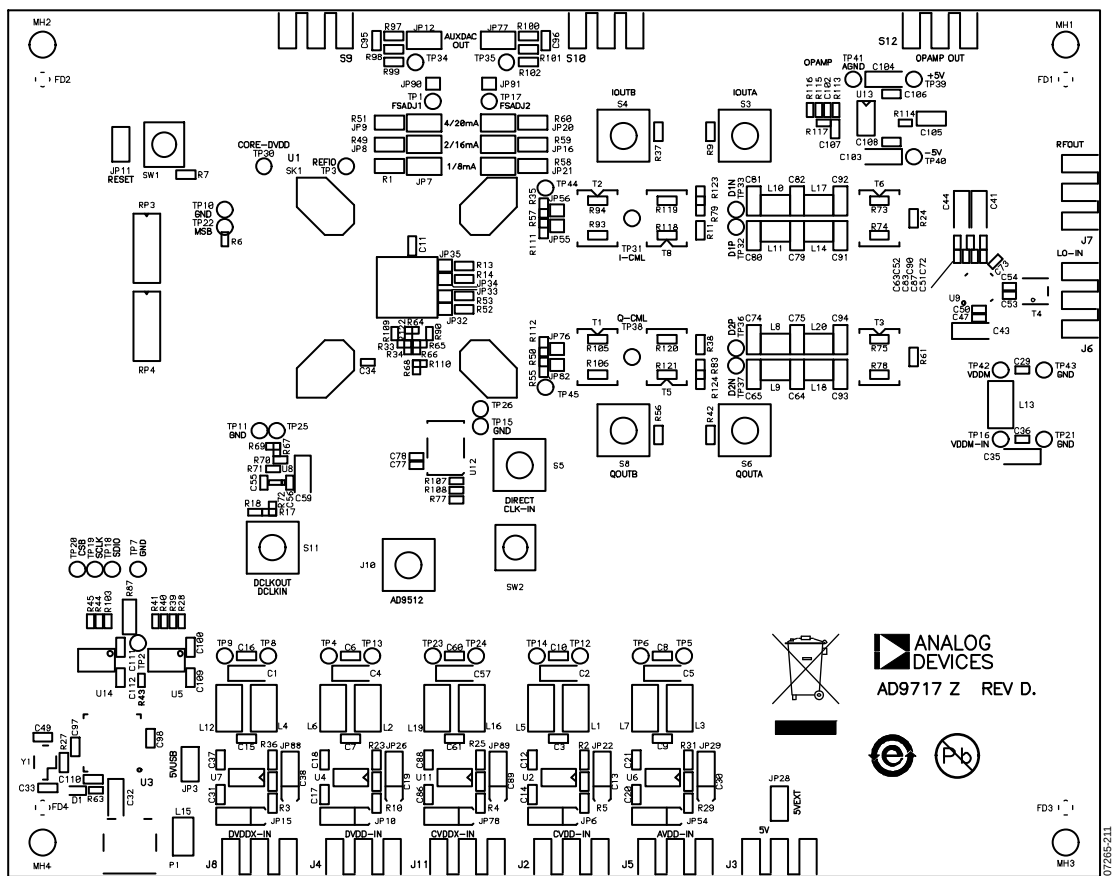
Figure 129. Silkscreen—Primary Side
