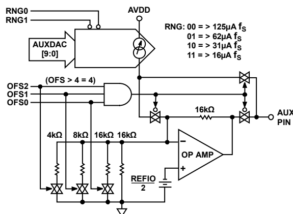
Figure 106. AUXDAC Simplified Circuit Diagram
