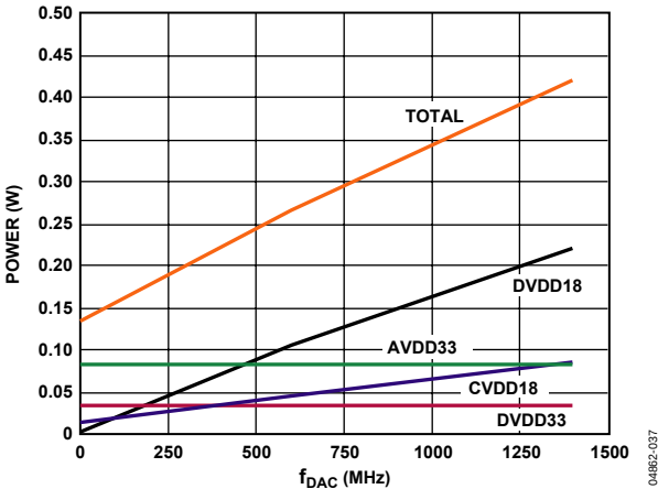
Figure 39. AD9736 1× Mode Power vs. f_{DAC} at 25°C
