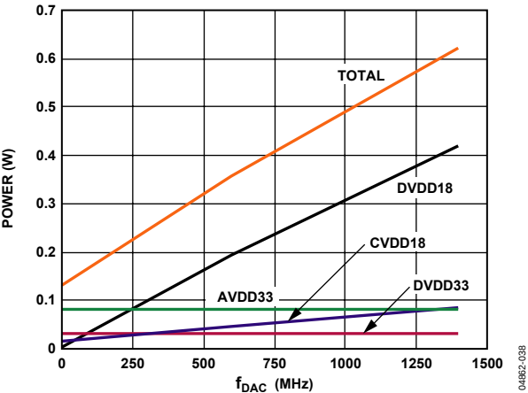
Figure 40. AD9736, 2× Interpolation Mode Power vs. f_{DAC} at 25°C
