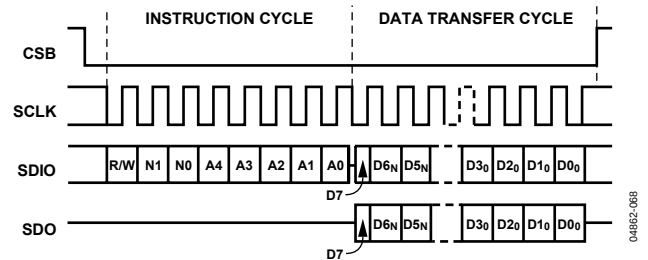
Figure 70. Serial Register Interface Timing, MSB-First Read
