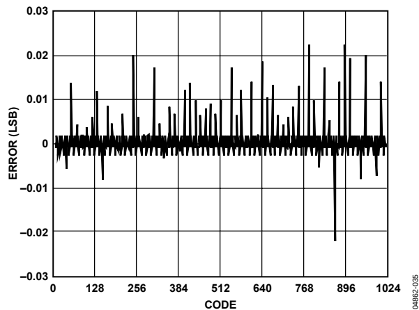
Figure 37. AD9734 DNL, 25°C, 20 mA FS
