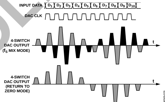
Figure 35. Mix Mode and RZ Mode DAC Waveforms
