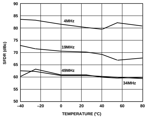
Figure 17. SFDR vs. Temperature @ 165 MSPS, 0 dBFS
