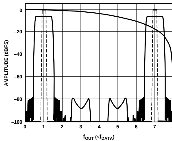
Figure 74. 8× Interpolation, Modulation = f_{DAC}/8
