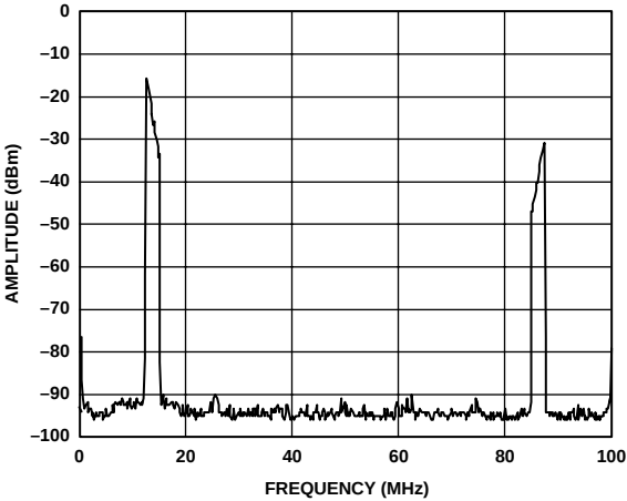
Figure 95. AD9775 Real DAC Output of Complex Input Signal Near Baseband (Positive Frequencies Only), Interpolation = 8 \times , Complex Modulation in AD9775 = +f_{DAC}/8
