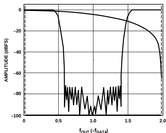
Figure 63. 2× Interpolation, Modulation = Disabled
