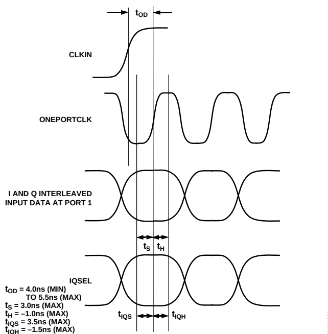
Figure 56. Timing Requirements in One-Port Input Mode with PLL Disabled
