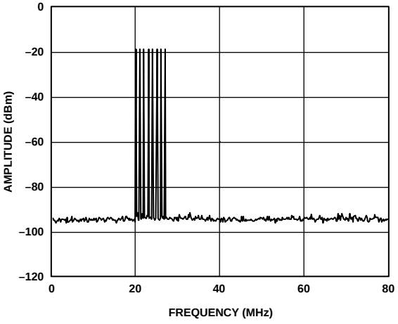
Figure 31. Eight-Tone IMD Performance, f_{DATA} = 160\text{ MSPS} , Interpolation = 8x
