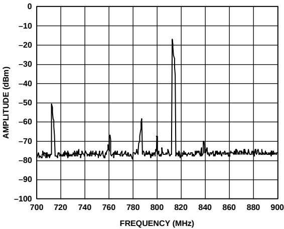
Figure 96. AD9775 Complex Output from Figure 95, Now Quadrature Modulated by AD8345 (LO = 800 MHz)
