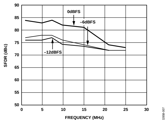
Figure 7. In-Band SFDR vs. f_{\text{OUT}} @ f_{\text{DATA}} = 65\text{ MSPS}
