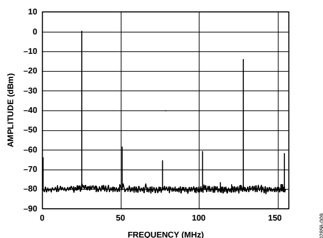
Figure 9. Single-Tone Spectrum @ f_{\text{DATA}} = 78\text{ MSPS} with f_{\text{OUT}} = f_{\text{DATA}}/3
