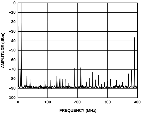
Figure 30. Single-Tone Spurious Performance, f_{OUT} = 10\text{ MHz} , f_{DATA} = 50\text{ MSPS} , Interpolation = 8x
