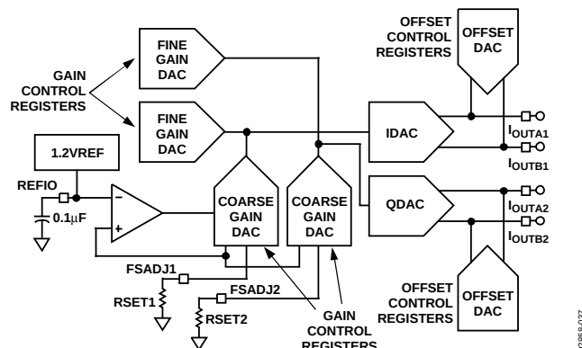
Figure 37. DAC Outputs, Reference Current Scaling, and Gain/Offset Adjust
