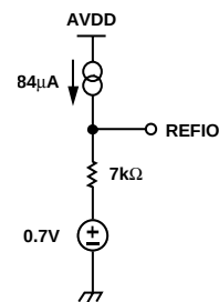
Figure 38. Equivalent Internal Reference Circuit
