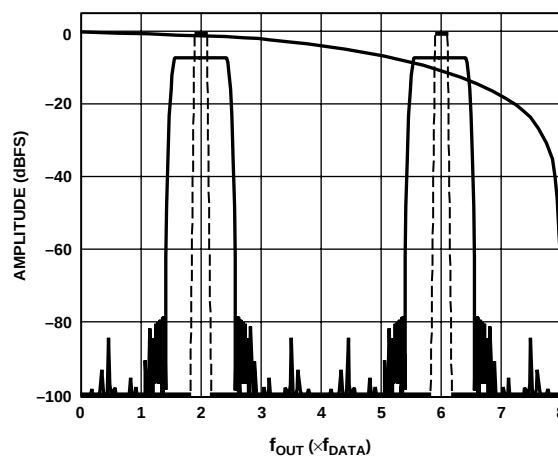
Figure 73. 8× Interpolation, Modulation = f_{DAC}/4
