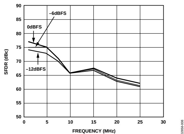
Figure 8. Out-of-Band SFDR vs. f_{\text{OUT}} @ f_{\text{DATA}} = 65\text{ MSPS}
