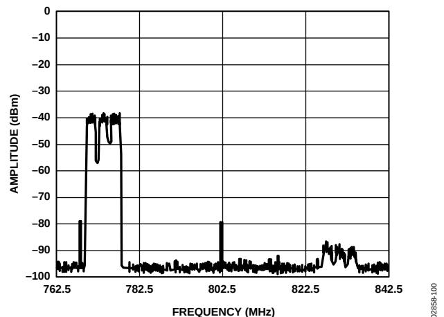
Figure 100. AD9775/AD8345 Synthesizing a Three-Carrier WCDMA Signal at an LO of 800 MHz
