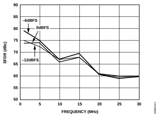
Figure 11. Out-of-Band SFDR vs. f_{\text{OUT}} @ f_{\text{DATA}} = 78\text{ MSPS}
