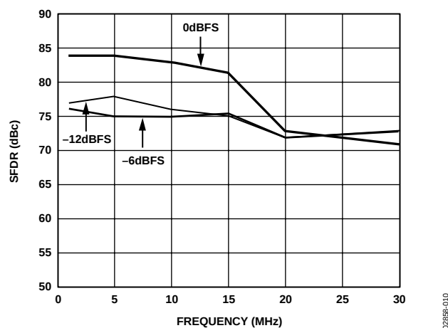
Figure 10. In-Band SFDR vs. f_{\text{OUT}} @ f_{\text{DATA}} = 78\text{ MSPS}
