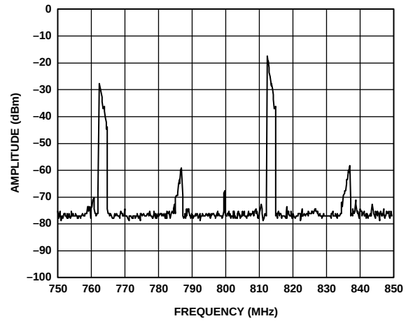
Figure 92. AD9775 Complex Output from Figure 91, Now Quadrature Modulated by AD8345 (LO = 800 MHz)
