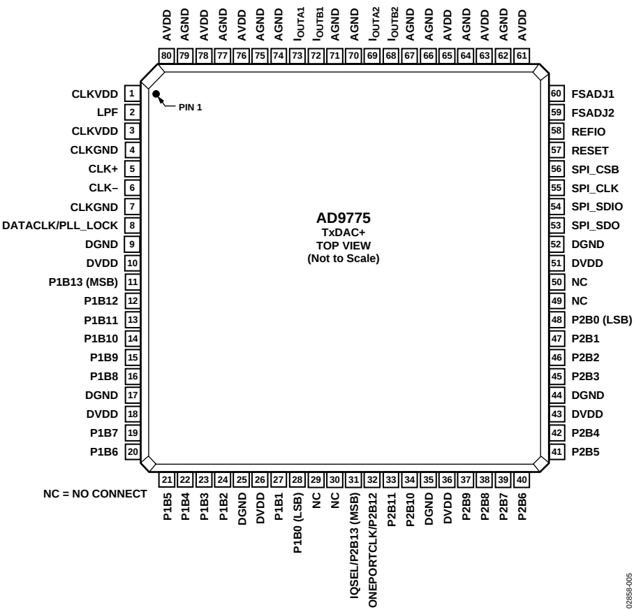
Figure 5. Pin Configuration
