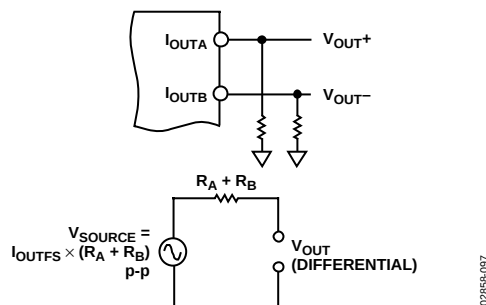
Figure 97. DAC Output Equivalent Circuit
