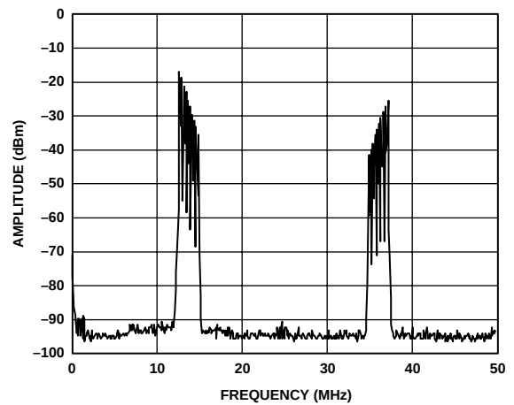
Figure 93. AD9775 Real DAC Output of Complex Input Signal Near Baseband (Negative Frequencies Only), Interpolation = 4x, Complex Modulation in AD9775 = -f_{DAC}/4
