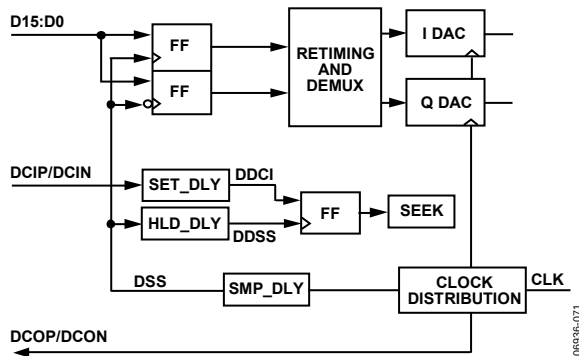
Figure 56. Digital Data Port Block Diagram
