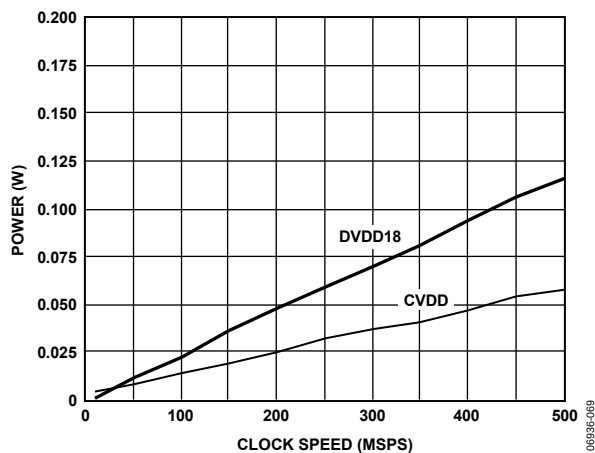
Figure 72. Power Dissipation, Digital 1.8 V Supply, Clock 1.8 V Supply, I and Q Data, Dual DAC Mode
