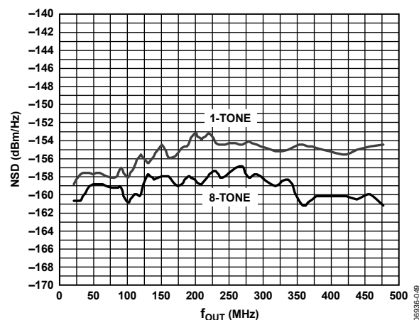
Figure 49. AD9780 One-Tone, Eight-Tone NSD vs. f_{OUT} in Baseband and Mix Modes, at 500 MSPS, FS = 20 mA
