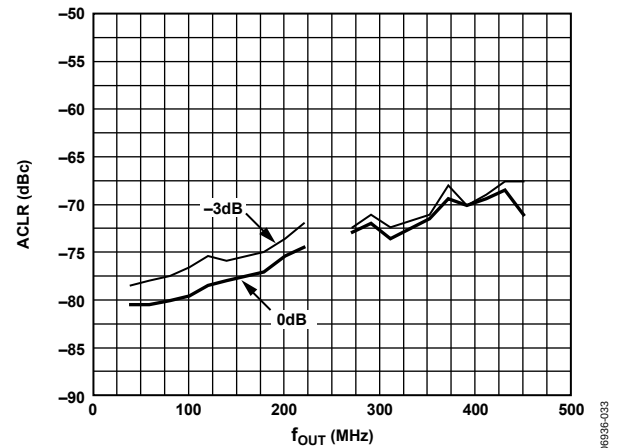
Figure 33. AD9783 ACLR for Second Adjacent Channel Two-Carrier W-CDMA Over Digital Input Level Baseband and Mix Modes, at 491.52 MSPS, FS = 20 mA
