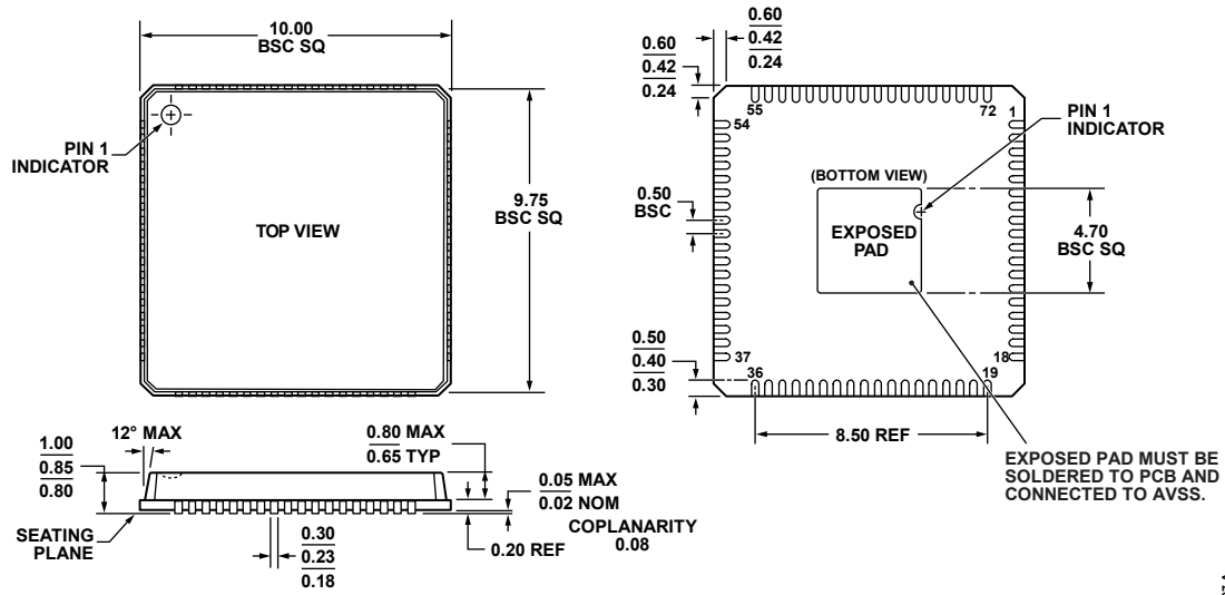
Figure 79. 72-Lead Lead Frame Chip Scale Package [LFCSP_VQ] 10 mm × 10 mm, Very Thin Quad (CP-72-1) Dimensions shown in millimeters
