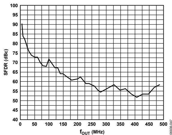
Figure 47. AD9780 SFDR vs. f_{OUT} in Baseband and Mix Modes, at 500 MSPS, FS = 20 mA
