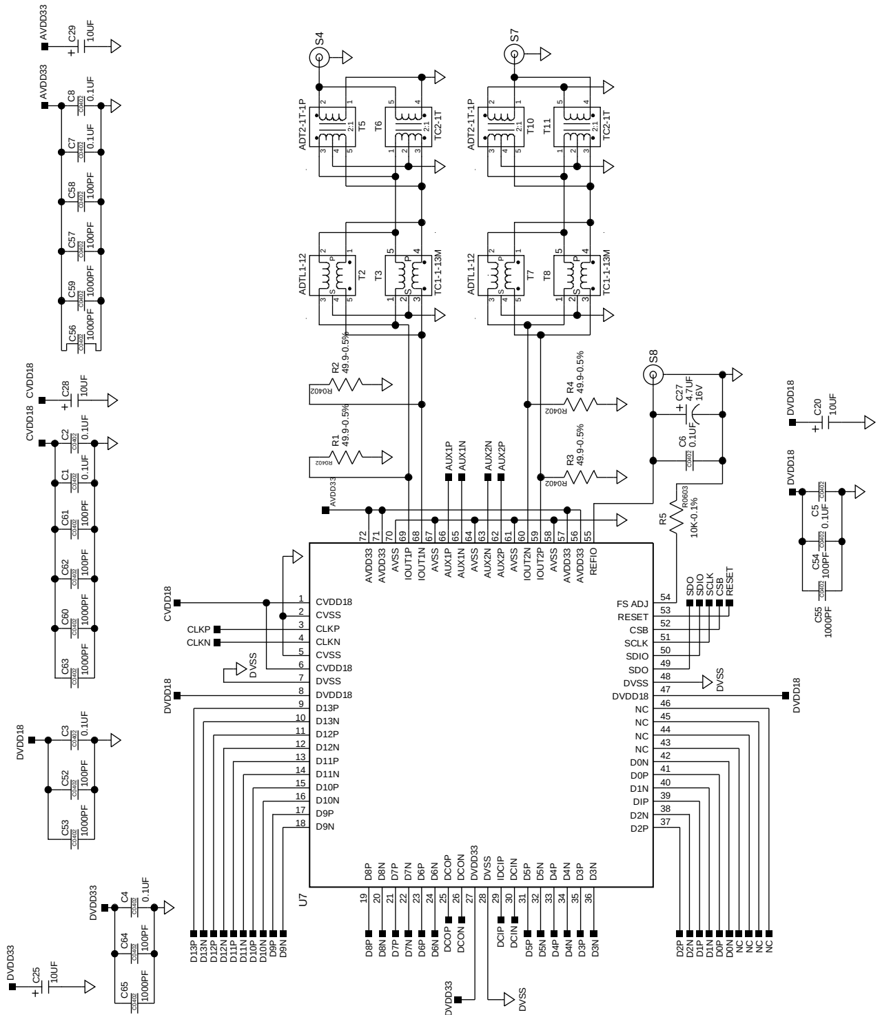
Figure 76. Main Schematic
