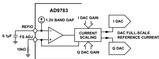
Figure 62. Reference Circuitry
