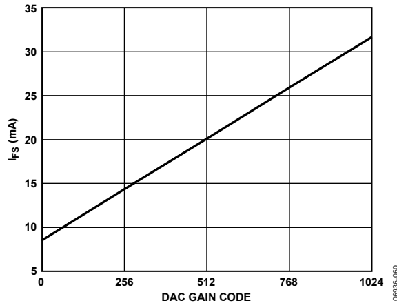
Figure 63. I_{FS} vs. DAC Gain Code
