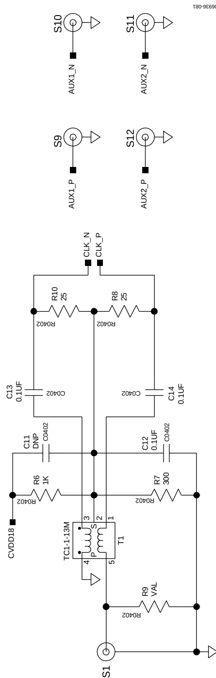
Figure 78. AUX DAC and Clock Input Circuit Details
