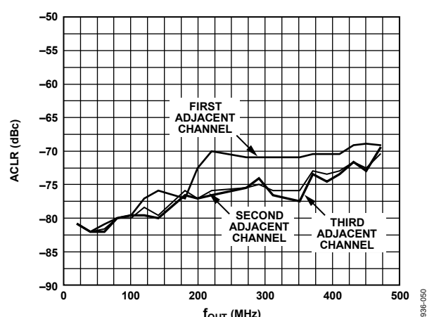
Figure 50. AD9780 ACLR for One-Carrier W-CDMA Baseband and Mix Modes, at 491.52 MSPS, FS = 20 mA
