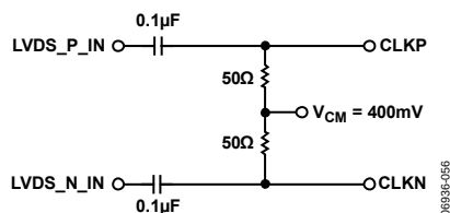
Figure 59. LVDS DAC CLK Drive Circuit
