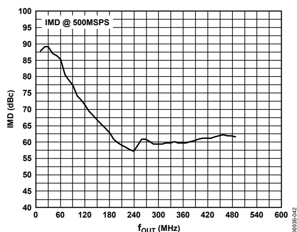
Figure 42. AD9781 IMD vs. f_{OUT} in Baseband and Mix Modes, at 500 MSPS, FS = 20 mA
