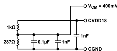
Figure 61. DAC CLK VCM Generator Circuit
