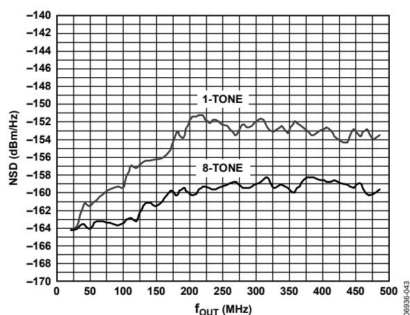
Figure 43. AD9781 One-Tone, Eight-Tone NSD vs. f_{OUT} in Baseband and Mix Modes, at 500 MSPS, FS = 20 mA
