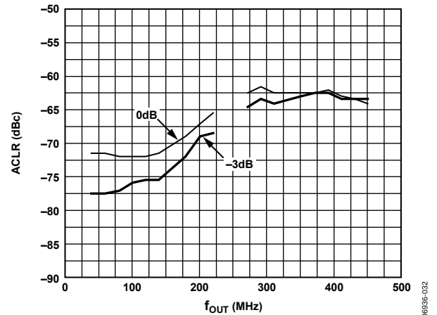
Figure 32. AD9783 ACLR for First Adjacent Channel Two-Carrier W-CDMA Over Digital Input Level Baseband and Mix Modes, at 491.52 MSPS, FS = 20 mA
