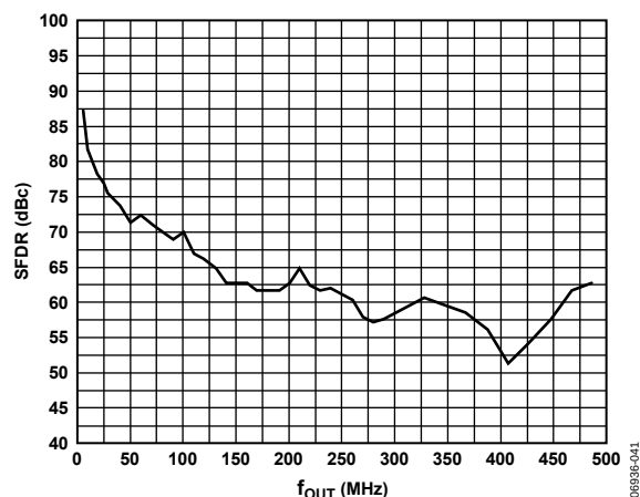
Figure 41. AD9781 SFDR vs. f_{OUT} in Baseband and Mix Modes, at 500 MSPS, FS = 20 mA
