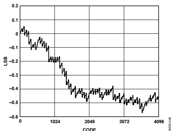
Figure 45. AD9780 INL, FS = 20 mA
