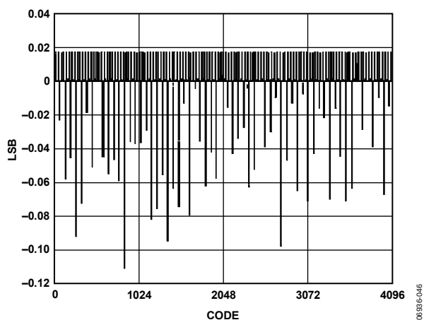
Figure 46. AD9780 DNL, FS = 20 mA
