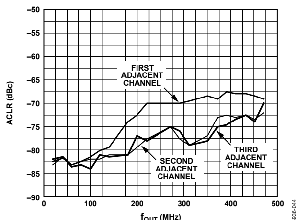
Figure 44. AD9781 ACLR for One-Carrier W-CDMA Baseband and Mix Modes, at 491.52 MSPS, FS = 20 mA
