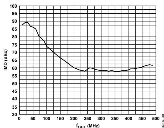
Figure 48. AD9780 IMD vs. f_{OUT} in Baseband and Mix Modes, at 500 MSPS, FS = 20 mA
