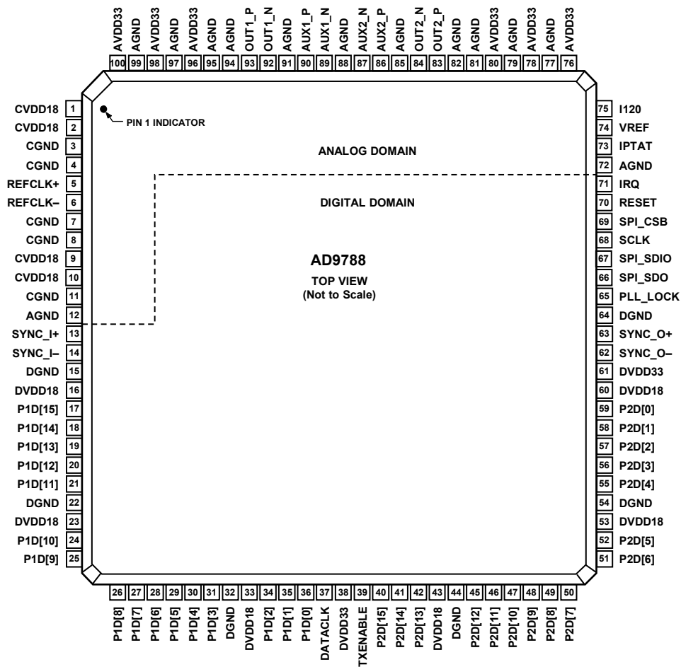
Figure 4. AD9788 Pin Configuration
