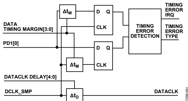
Figure 52. Timing Error Detection and Optimization Circuitry
