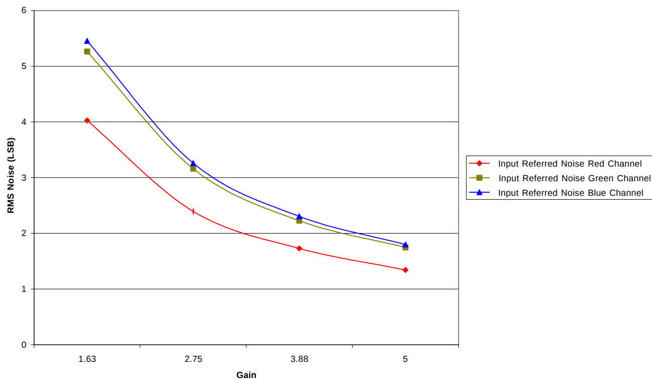
Graph 6. XRD9814B 3-Channel CDS Pixel Clamp Input Referred Noise vs. Gain
