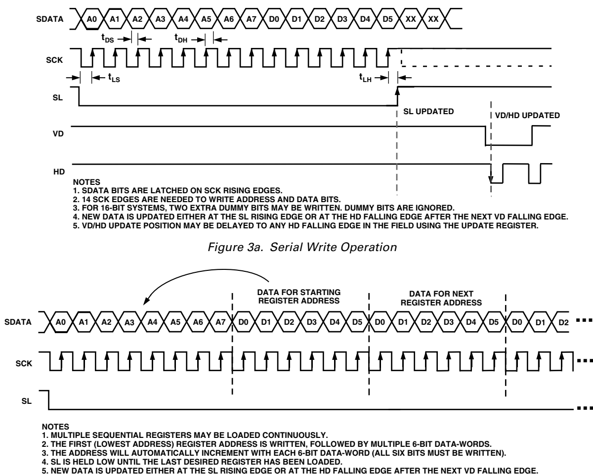
Figure 3b. Continuous Serial Write Operation
