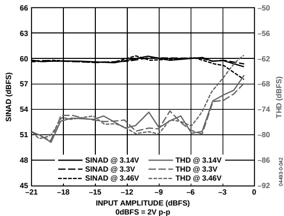
Figure 5. SINAD and THD vs. Input Amplitude and Supply ( f_{\text{IN}} = 8 MHz, LPF f_{-3\text{dB}} = 26 MHz; R_{\text{xPGA}} = 0 dB)
