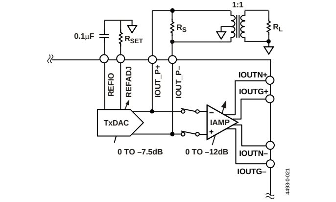
Figure 63. TxDAC Output Directly via Center-Tap Transformer
