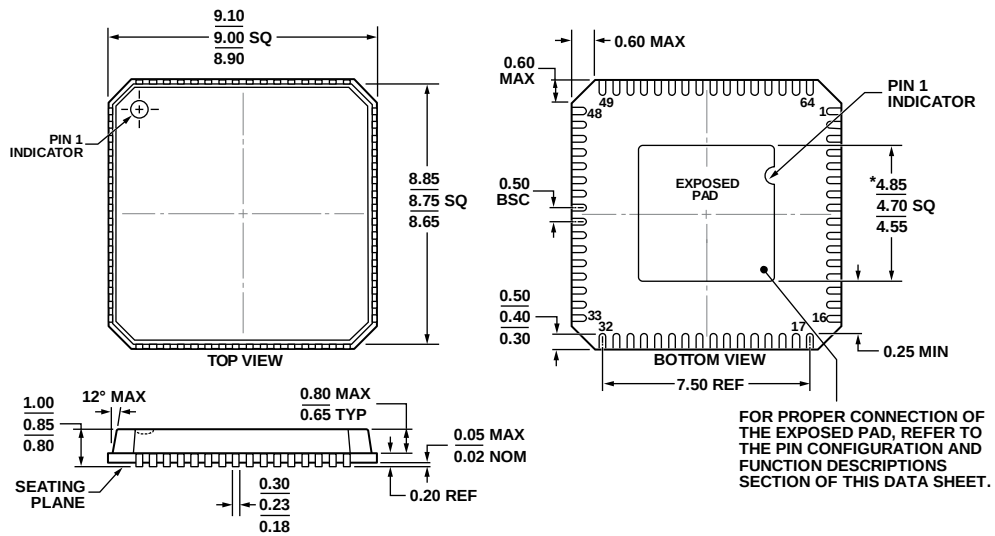
*COMPLIANT TO JEDEC STANDARDS MO-220-VMM4 EXCEPT FOR EXPOSED PAD DIMENSION Figure 6. 64-Lead Lead Frame Chip Scale Package [LFCSP_VQ] 9 mm × 9 mm Body, Very Thin Quad (CP-64-1) Dimensions shown in millimeters
