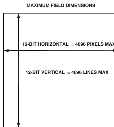
Figure 2a. Vertical and Horizontal Counters
