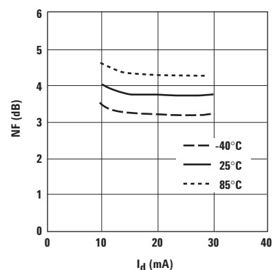
Figure 11. NF vs. I_d and Temperature at 900 MHz.
