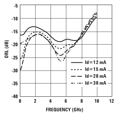
Figure 17. Output Return Loss vs. I_d and Frequency (GHz).
