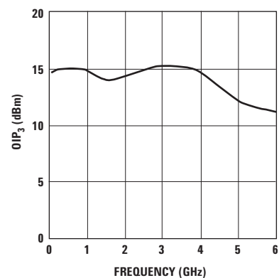
Figure 5. OIP_3 vs. Frequency at I_d = 15 mA.
