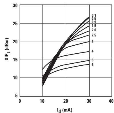
Figure 14. OIP_3 vs. I_d and Frequency (GHz).
