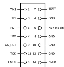
14-pin TI-style JTAG pinout
