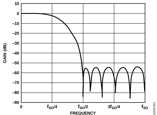
Figure 21. Decimation Filter Transfer Function, f_{SI} = 800 \text{ kHz}
