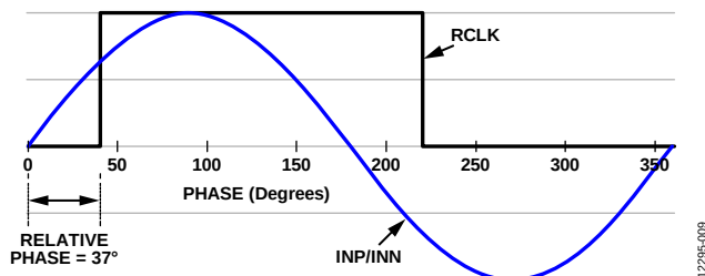
Figure 14. Example Showing Relative Phase, \theta_{REL} , of 37^\circ
