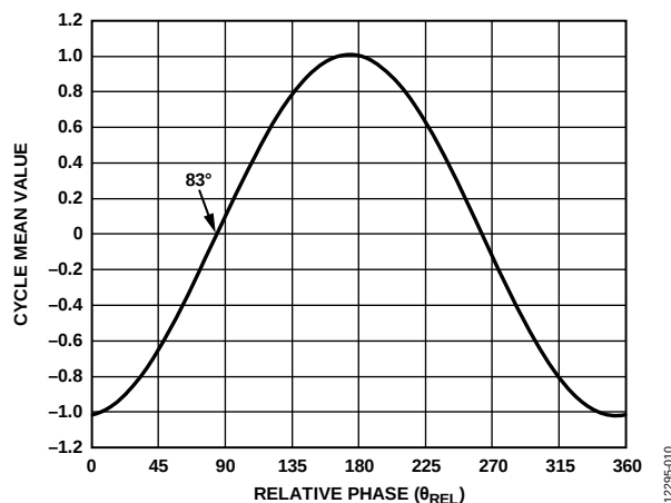
Figure 15. Phase Transfer Function with Phase Delay of 83^\circ , 1 V rms Input
