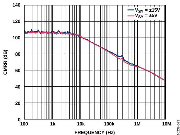
Figure 38. CMRR vs. Frequency, V_{SV} = \pm 5V and V_{SV} = \pm 15V
