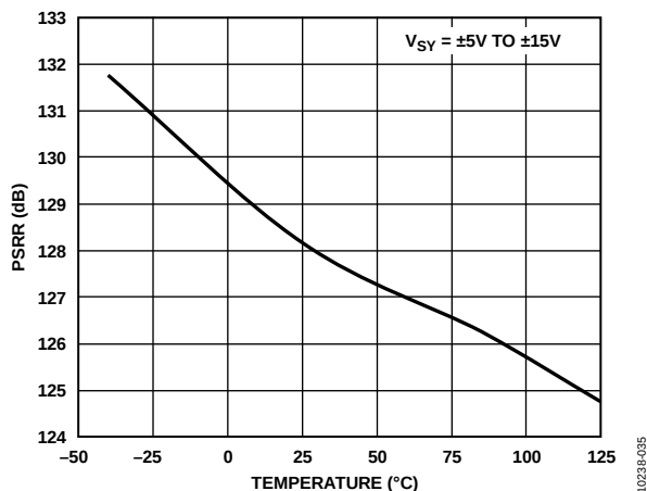
Figure 35. PSRR vs. Temperature, V_{SV} = \pm 5V to \pm 15V
