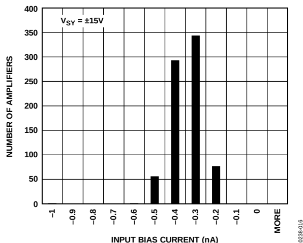
Figure 27. Input Bias Current, V_{SY} = \pm 15 V
