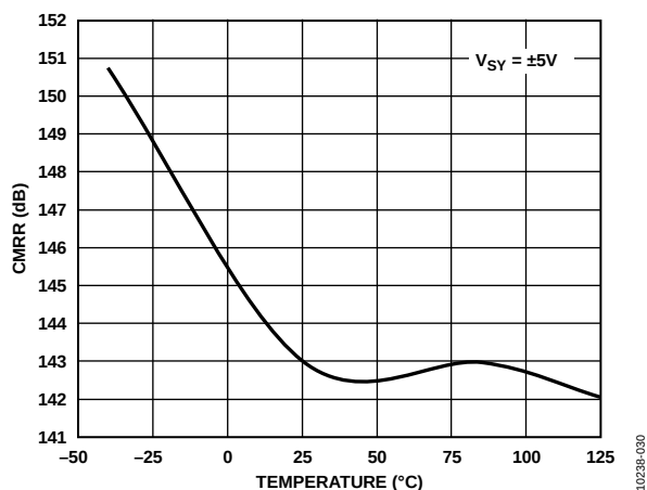
Figure 37. CMRR vs. Temperature, V_{SV} = \pm 5V
