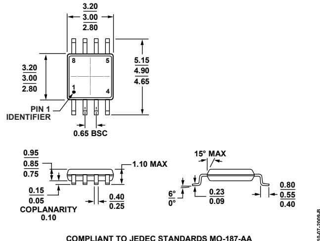
Figure 71. 8-Lead Mini Small Outline Package [MSOP]
