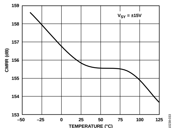
Figure 40. CMRR vs. Temperature, V_{SV} = \pm 15V
