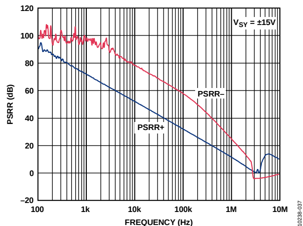
Figure 39. PSRR vs. Frequency, V_{SV} = \pm 15V
