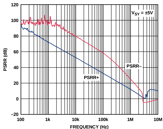
Figure 36. PSRR vs. Frequency, V_{SV} = \pm 5V
