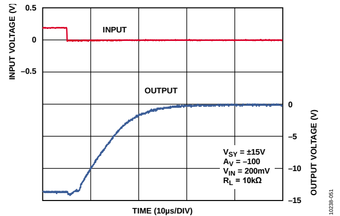
Figure 52. Negative Overload Recovery, V_{SY} = \pm 15\text{ V}
