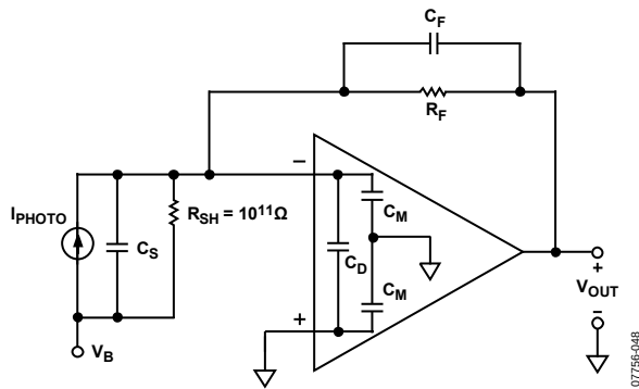
Figure 50. Wideband Photodiode Preamplifier
