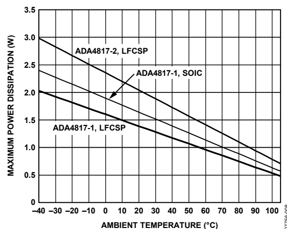
Figure 4. Maximum Safe Power Dissipation vs. Ambient Temperature for a 4-Layer Board
