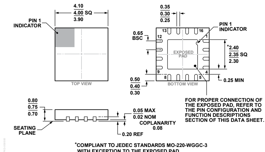
Figure 60. 16-Lead Lead Frame Chip Scale Package [LFCSP] 4 mm × 4 mm Body and 0.75 mm Package Height (CP-16-20)
