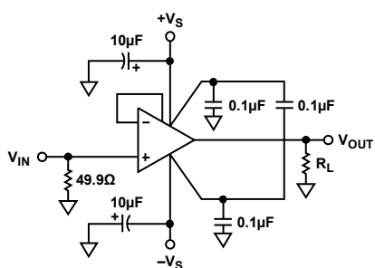
Figure 35. G = 1 Configuration
