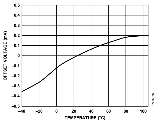
Figure 29. Offset Voltage vs. Temperature
