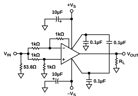
Figure 40. Common-Mode Rejection
