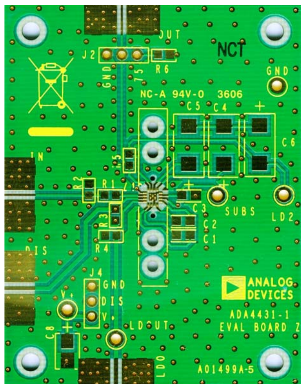
Figure 18. Evaluation Board—Front
