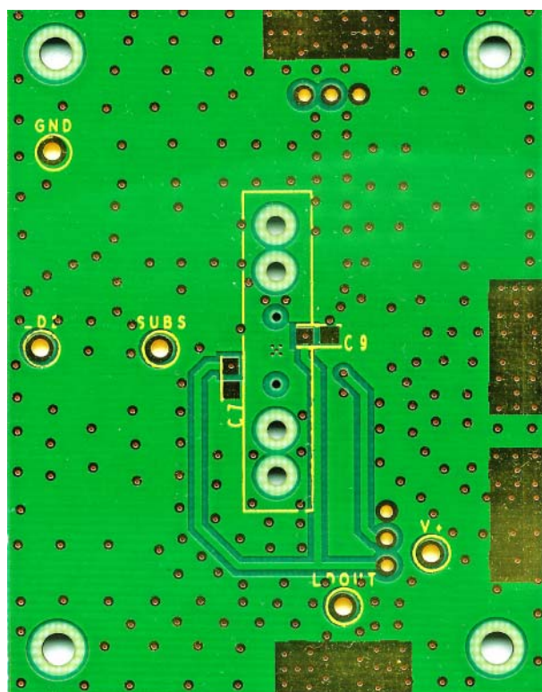
Figure 19. Evaluation Board—Back
