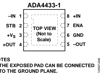
Figure 6. ADA4433-1 LFCSP Pin Configuration, Top View
