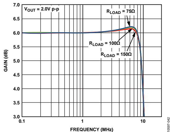
Figure 9. 1 dB Flatness Response at Various Load Resistances
