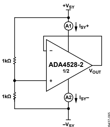
Figure 68. Voltage Follower
