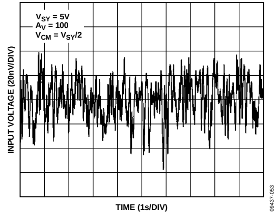
Figure 59. 0.1 Hz to 10 Hz Noise
