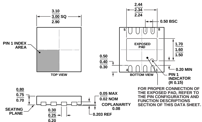
Figure 76. 8-Lead Lead Frame Chip Scale Package [LFCSP_WD] 3 mm × 3 mm Body, Very Very Thin, Dual Lead (CP-8-11) Dimensions shown in millimeters
