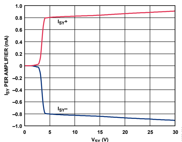
Figure 60. Supply Current vs. Supply Voltage (Voltage Follower)
