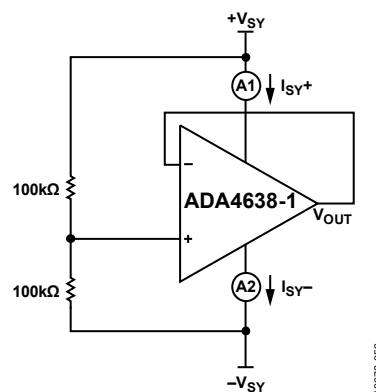
Figure 59. Voltage Follower
