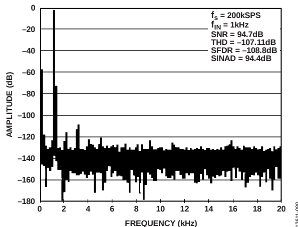
Figure 81. FFT for Driving a Single-Ended to Differential Converter Using Dynamic Power Scaling, -0.5 dBFS, On Time of 4 \mu s, for the Schematic Shown in Figure 76
