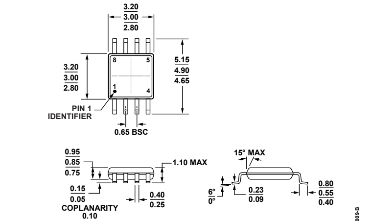
Figure 84. 8-Lead Mini Small Outline Package [MSOP] (RM-8)
