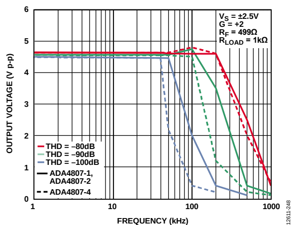
Figure 49. Output Voltage vs. Frequency for V_S = \pm 2.5\text{ V}
