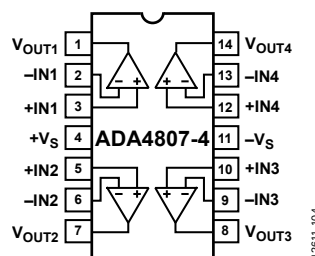
Figure 4. 14-Lead TSSOP Pin Configuration ( ADA4807-4 )
