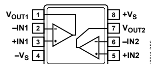
Figure 2. 8-Lead MSOP Pin Configuration ( ADA4807-2 )
