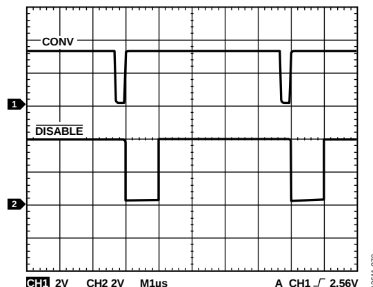
Figure 80. Dynamic Power Scaling Timing Diagram for Driving a Single-Ended Input Signal Chain into a Differential ADC (AD7982)
