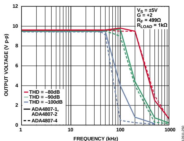
Figure 51. Output Voltage vs. Frequency for V_S = \pm 5\text{ V}
