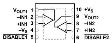
Figure 3. 10-Lead LFCSP Pin Configuration ( ADA4807-2 )
