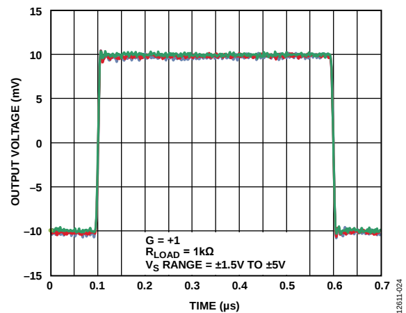
Figure 37. Small Signal Transient Response for Various Supplies
