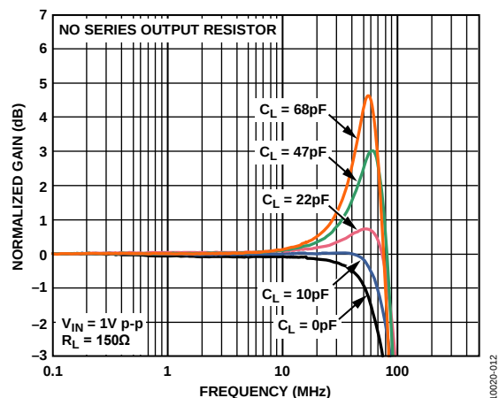
Figure 12. Large Signal Frequency Response for Various Capacitor Loads
