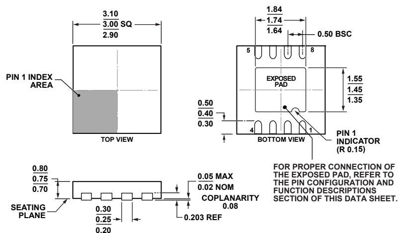
Figure 58. 8-Lead Lead Frame Chip Scale Package [LFCSP]
