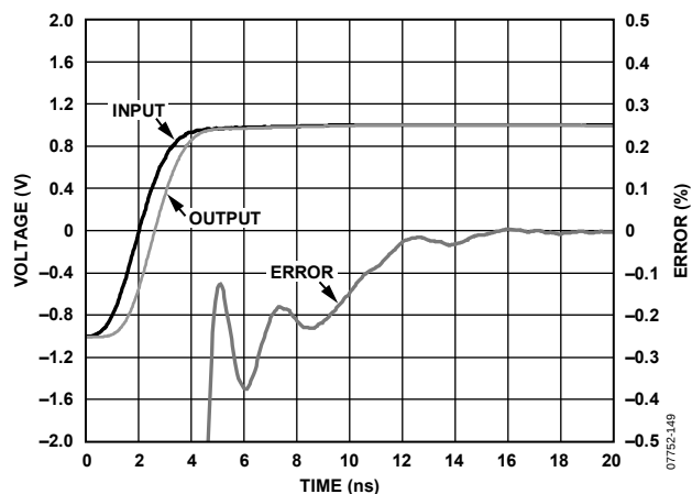
Figure 48. Settling Time
