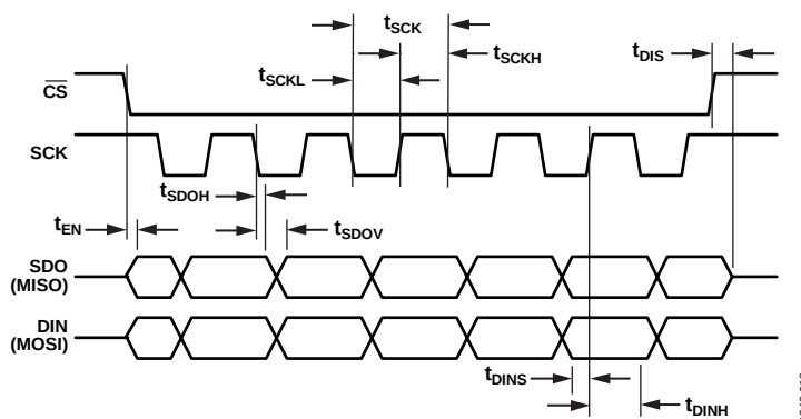
Figure 47. Serial Timing
