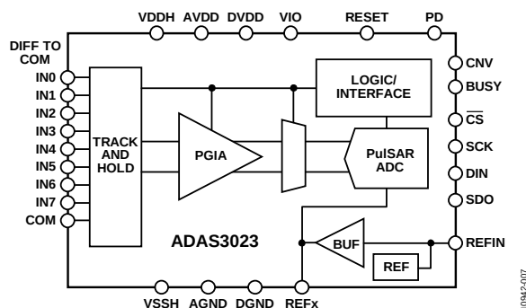
Figure 35. Simplified Block Diagram
