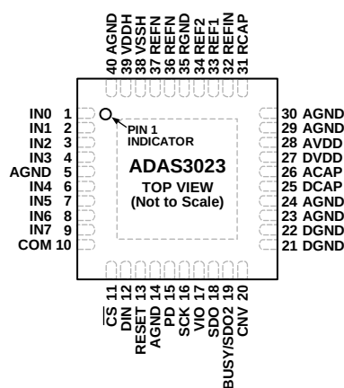
Figure 6. Pin Configuration
