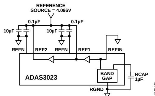
Figure 44. External Reference
