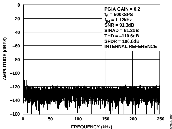
Figure 15. 1 kHz FFT, PGIA Gain = 0.2
