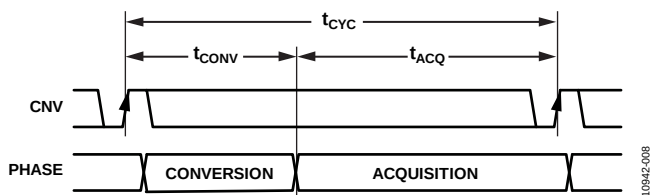
Figure 36. System Timing
