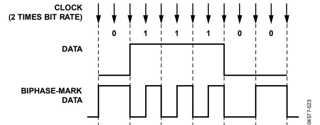
Figure 43. Biphase-Mark Encoding
