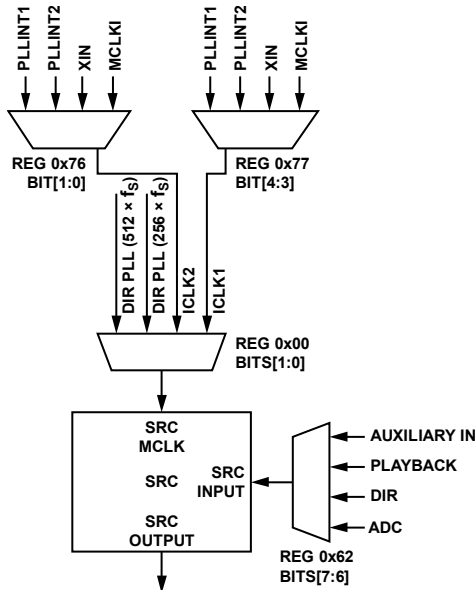
Figure 33. Clock and Datapath Control on the SRC
