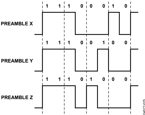
Figure 45. Preambles
