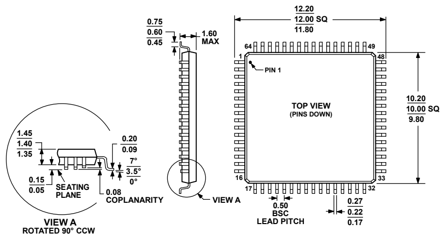
Figure 57. 64-Lead Low Profile Quad Flat Package [LQFP]
