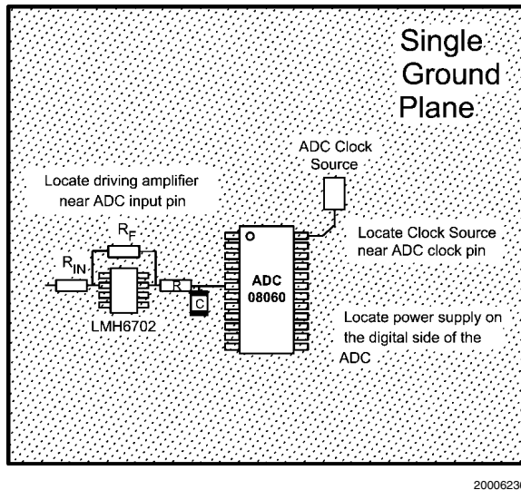
FIGURE 5. Layout Example
